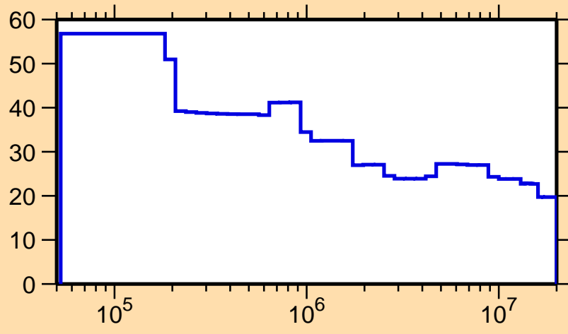
\Delta\sigma/\sigma vs. E for ^{247}\text{Cf}(n,n_1)
