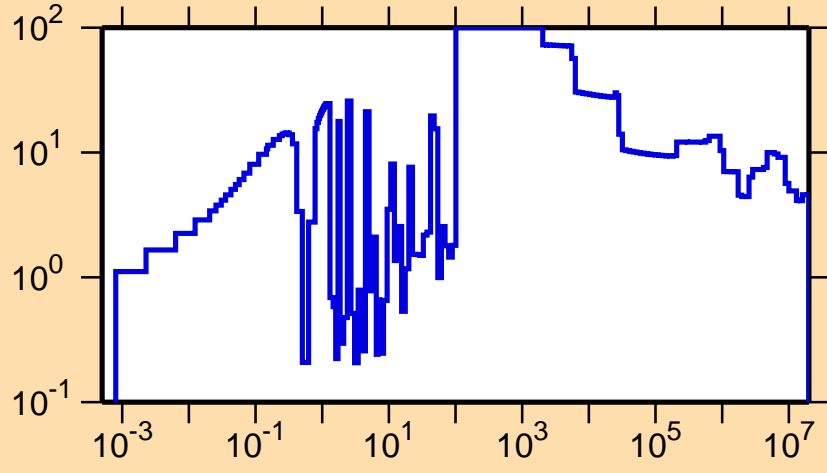
\Delta\sigma/\sigma vs. E for ^{247}\text{Cf}(n,\text{tot.})
