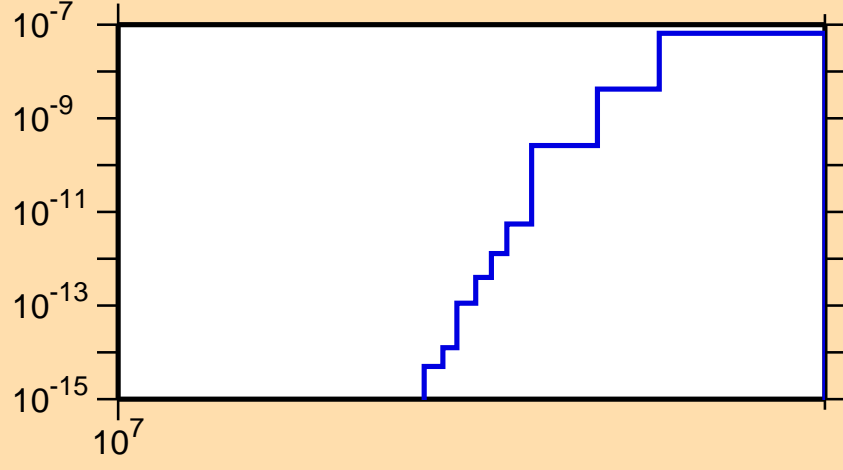
\sigma vs. E for ^{247}\text{Cf}(n,2np)
