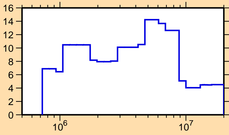
\Delta\sigma/\sigma vs. E for ^{247}\text{Cf}(n,el.)
