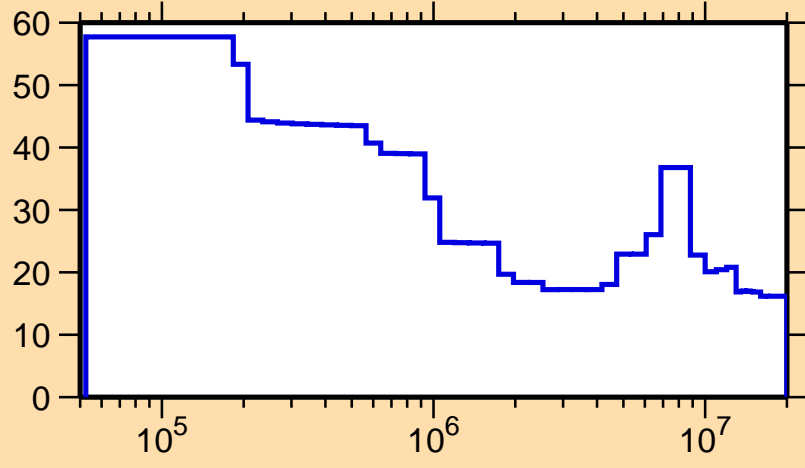
\Delta\sigma/\sigma vs. E for ^{247}\text{Cf}(n,\text{inel.})
