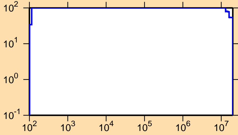
\Delta\sigma/\sigma vs. E for ^{247}\text{Cf}(n,f)
