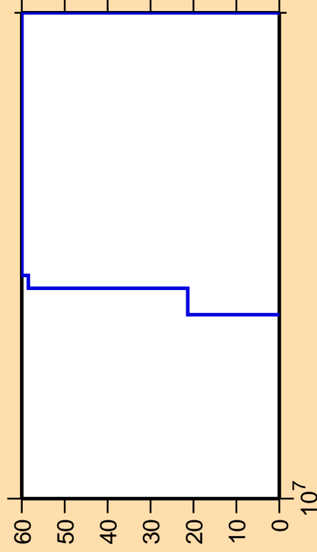
\Delta\sigma/\sigma vs. E for ^{247}\text{Cf}(\text{mt117})
