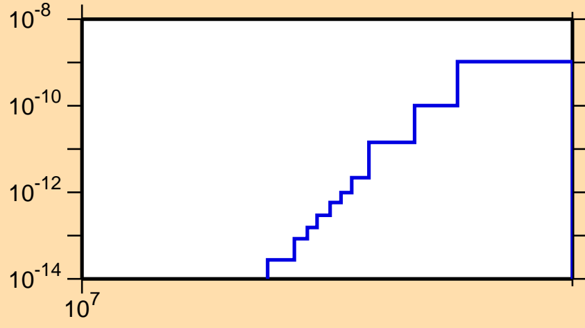
\sigma vs. E for ^{247}\text{Cf}(n,\text{He3})
