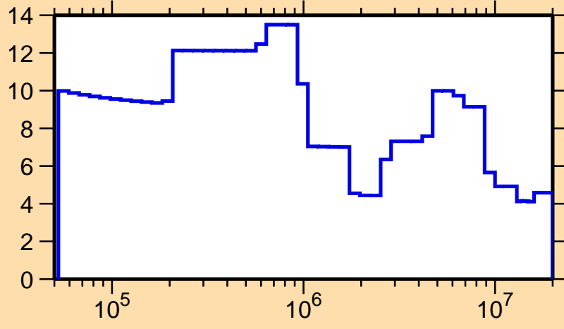
\Delta\sigma/\sigma vs. E for ^{247}\text{Cf}(n,\text{tot.})
