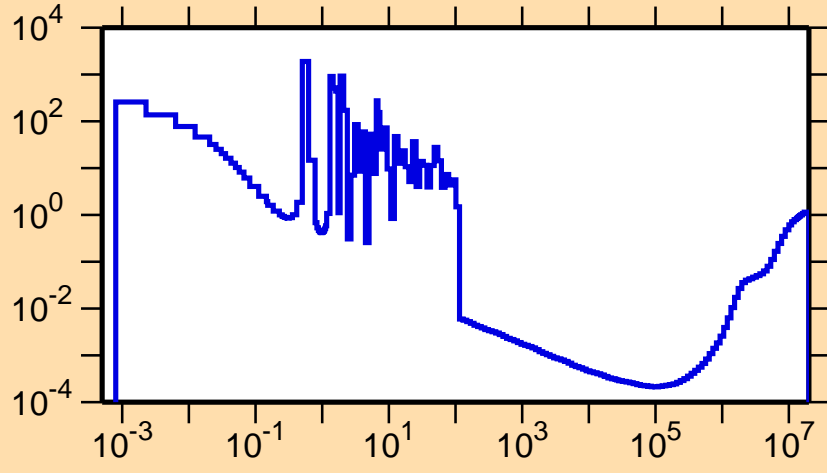
\sigma vs. E for ^{247}\text{Cf}(n,f)
