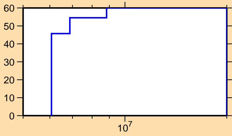
\Delta\sigma/\sigma vs. E for ^{247}\text{Cf}(n,2n)
