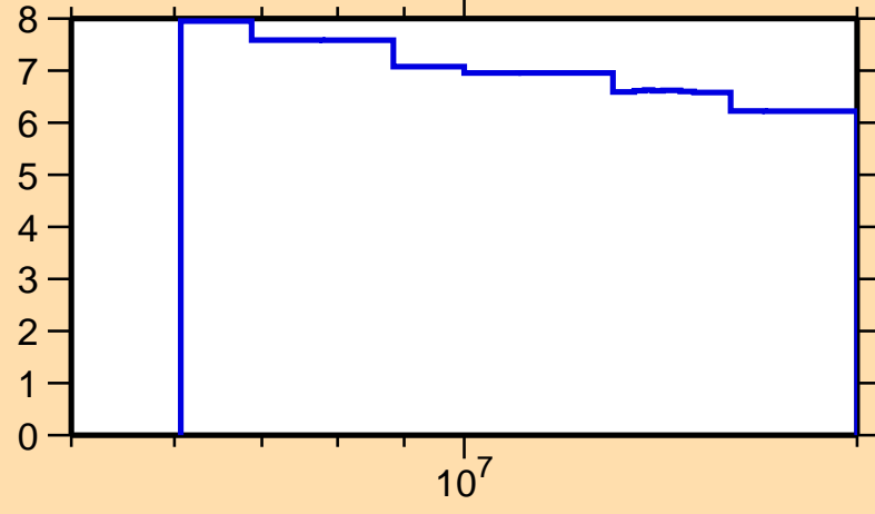
\Delta\sigma/\sigma vs. E for ^{247}\text{Cf}(n,\text{nonel.})
