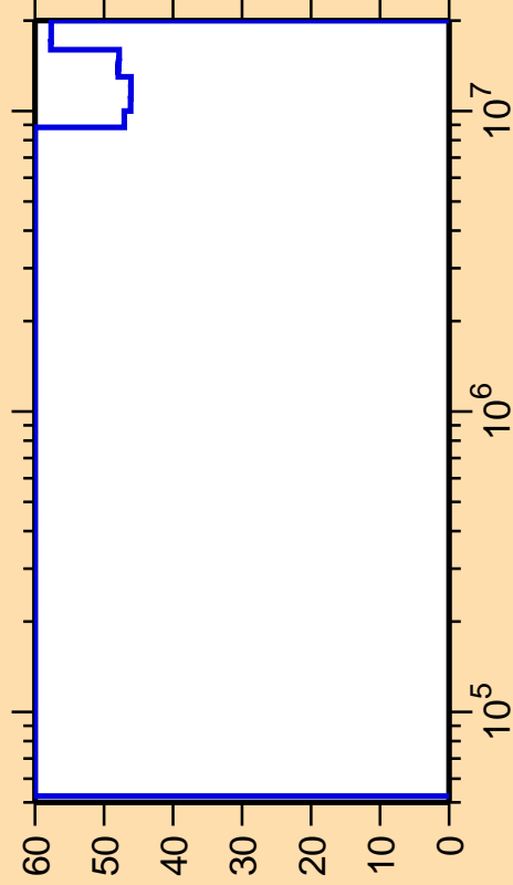
\Delta\sigma/\sigma vs. E for ^{247}\text{Cf}(n,\alpha)
