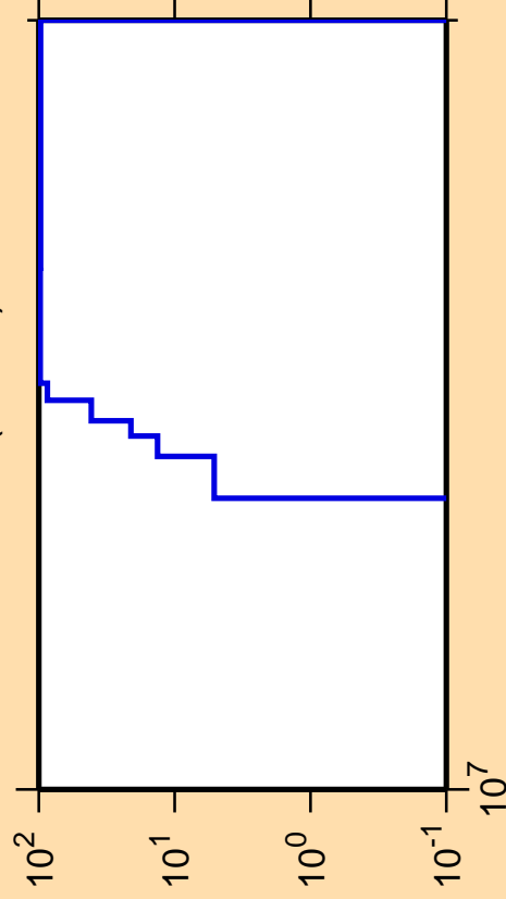
\Delta\sigma/\sigma vs. E for ^{247}\text{Cf} (mt 45)
