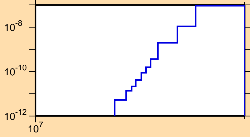
\sigma vs. E for ^{247}\text{Cf} (mt 45)
