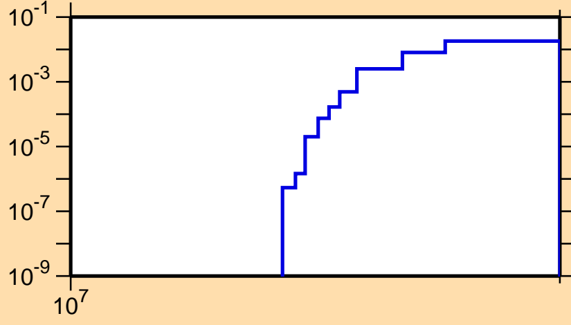
\sigma vs. E for ^{247}\text{Cf}(n,3n\alpha)
