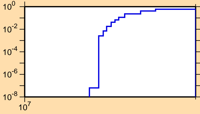
\sigma vs. E for ^{247}\text{Cf}(n,3n)
