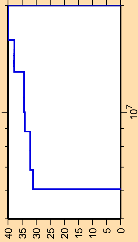
\Delta\sigma/\sigma vs. E for ^{247}\text{Cf}(n,p)
