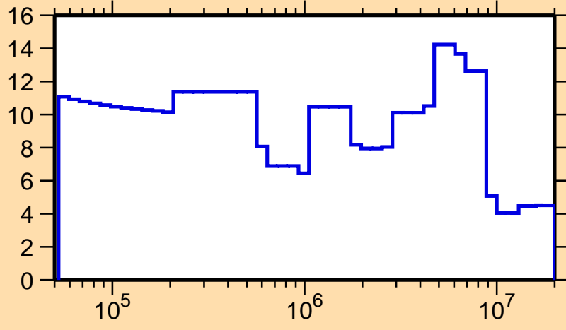
\Delta\sigma/\sigma vs. E for ^{247}\text{Cf}(n,\text{el.})
