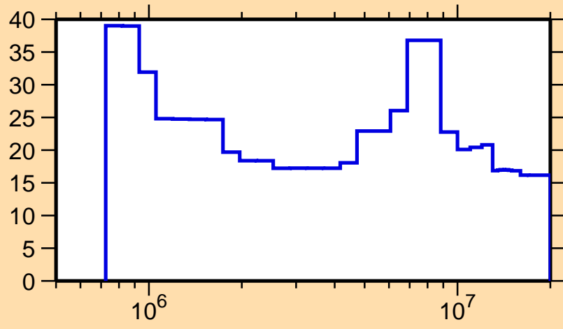
\Delta\sigma/\sigma vs. E for ^{247}\text{Cf}(n,\text{inel.})
