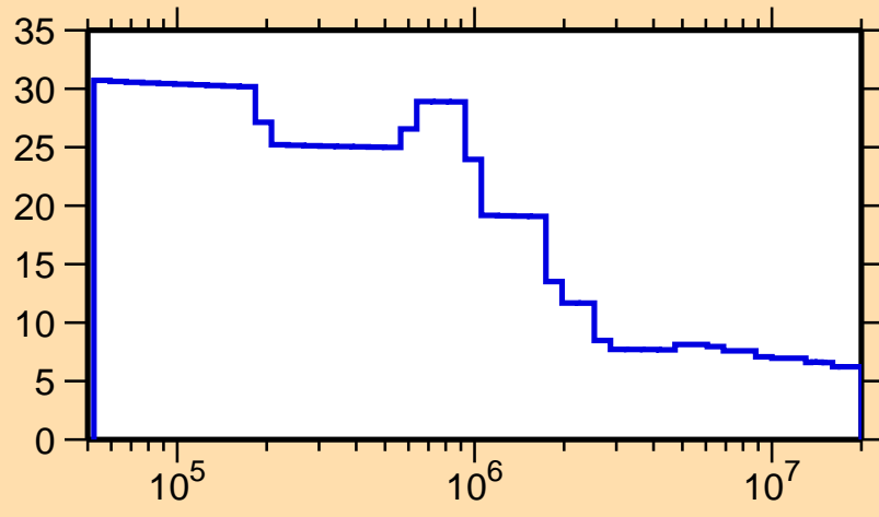
\Delta\sigma/\sigma vs. E for ^{247}\text{Cf}(n,\text{nonel.})
