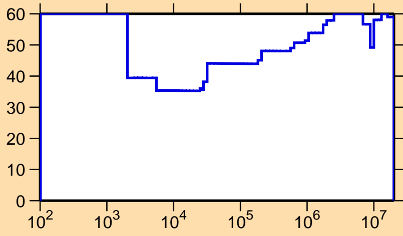
\Delta\sigma/\sigma vs. E for ^{247}\text{Cf}(n,\gamma)
