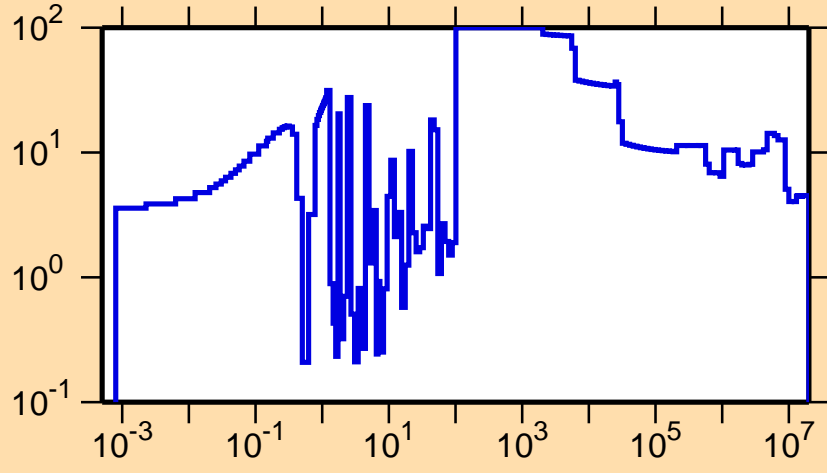
\Delta\sigma/\sigma vs. E for ^{247}\text{Cf}(n,\text{el.})
