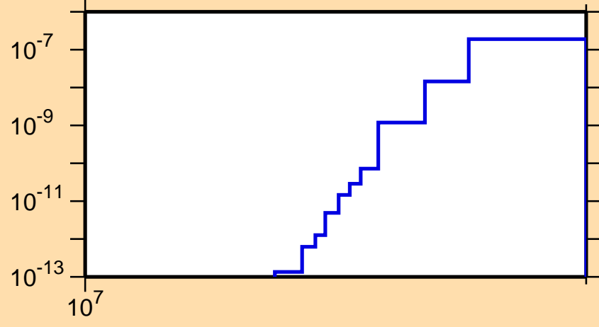
\sigma vs. E for ^{247}\text{Cf}(n,nd)
