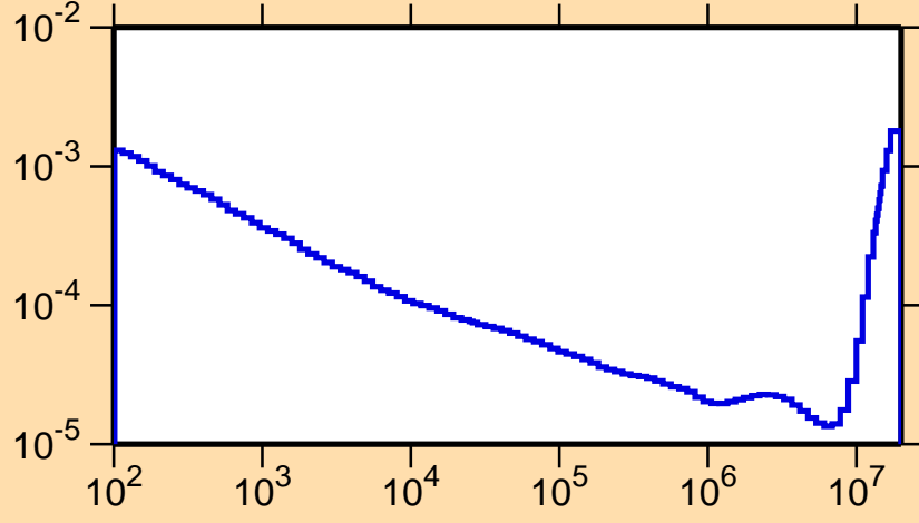
\sigma vs. E for ^{247}\text{Cf}(n,\alpha)
