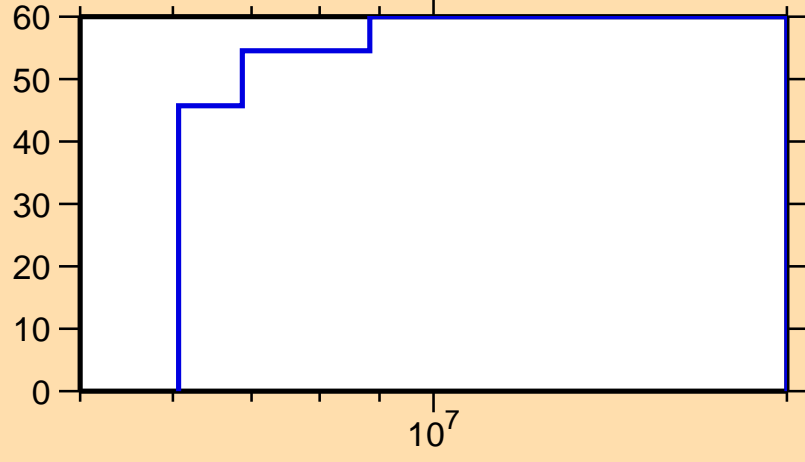
\Delta\sigma/\sigma vs. E for ^{247}\text{Cf}(n,2n)
