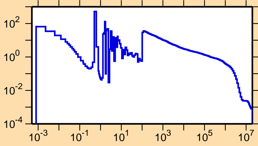
\sigma vs. E for ^{247}\text{Cf}(n,\gamma)
