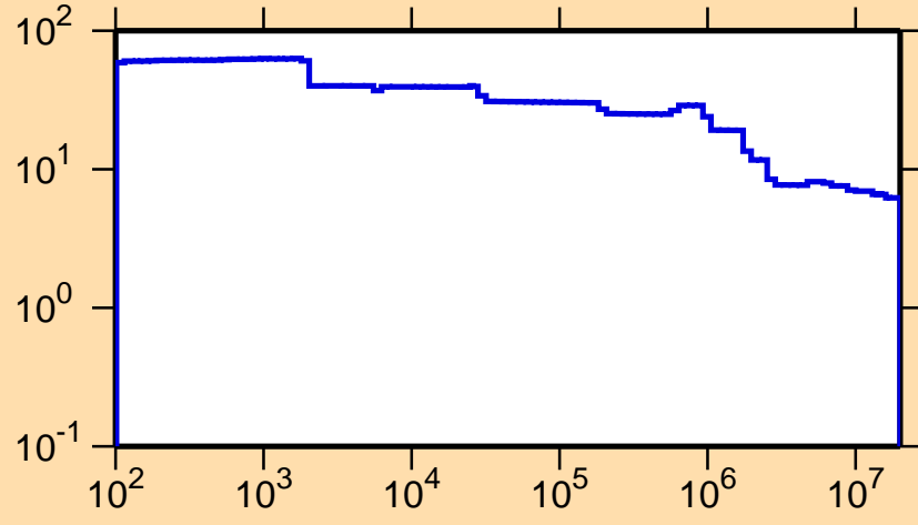
\Delta\sigma/\sigma vs. E for ^{247}\text{Cf}(n,\text{nonel.})
