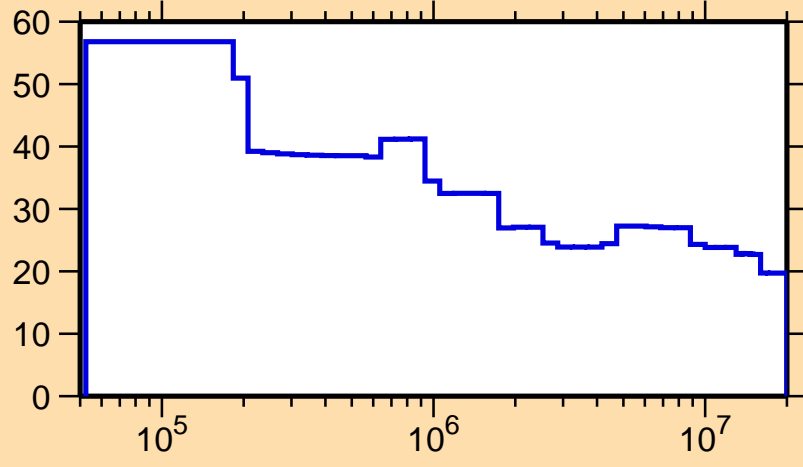
\Delta\sigma/\sigma vs. E for ^{247}\text{Cf}(n,n_1)
