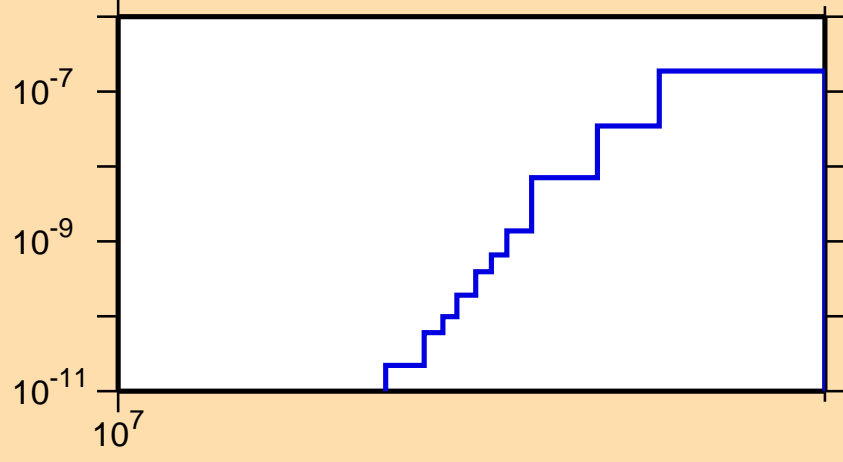
\sigma vs. E for ^{247}\text{Cf}(\text{mt117})
