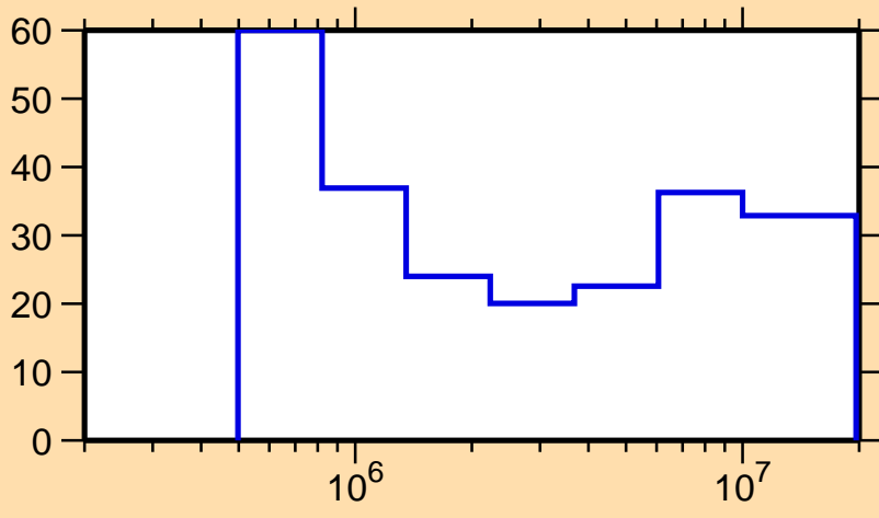
\Delta\sigma/\sigma vs. E for ^{247}\text{Cf}(n,n\text{cont.})
