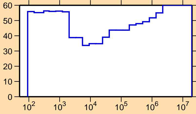
\Delta\sigma/\sigma vs. E for ^{247}\text{Cf}(n,\gamma)
