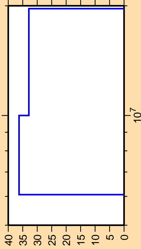
\Delta\sigma/\sigma vs. E for ^{247}\text{Cf}(n,n\text{cont.})
