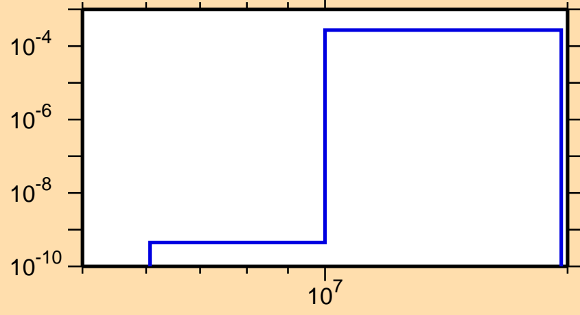
\sigma vs. E for ^{247}\text{Cf}(n,d)
