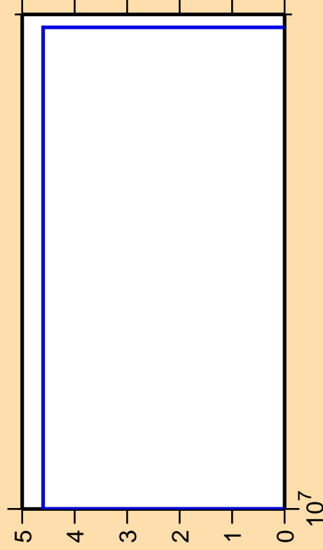
\Delta\sigma/\sigma vs. E for ^{247}\text{Cf}(n,\text{He3})
