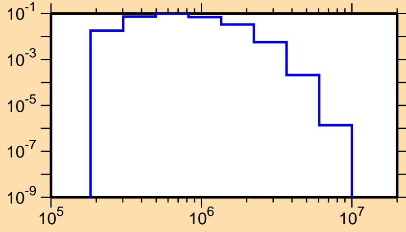
\sigma vs. E for ^{247}\text{Cf}(n,n_3)
