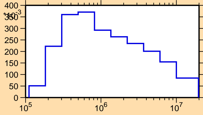
\sigma vs. E for ^{247}\text{Cf}(n,n_2)
