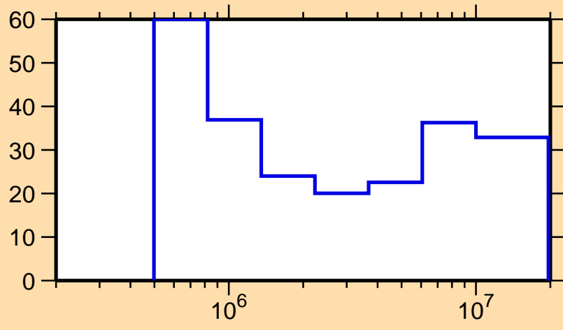
\Delta\sigma/\sigma vs. E for ^{247}\text{Cf}(n, ncont.)
