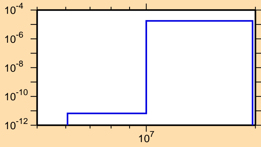
\sigma vs. E for ^{247}\text{Cf}(n,t)
