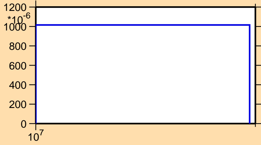
\sigma vs. E for ^{247}\text{Cf}(n,3n\alpha)
