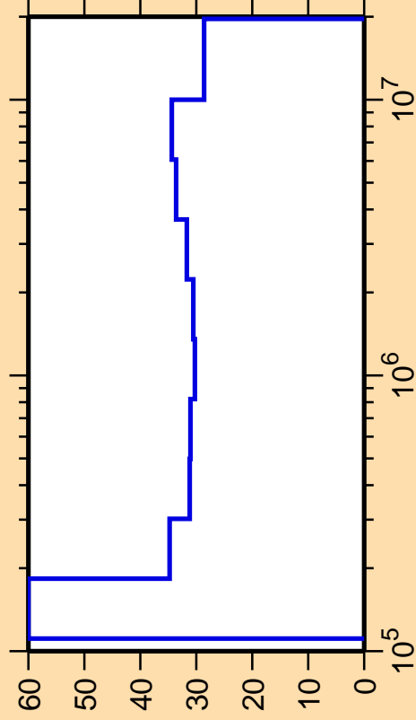
\Delta\sigma/\sigma vs. E for ^{247}\text{Cf}(n,n_2)
