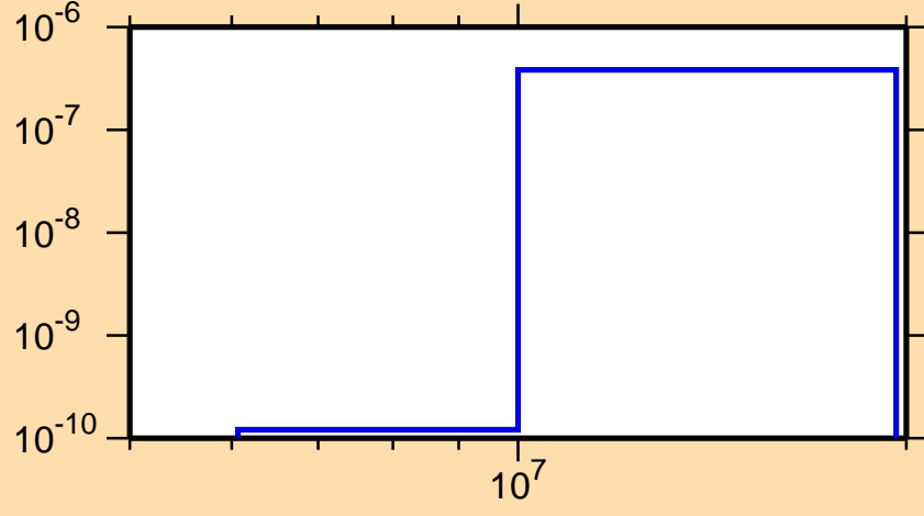
\sigma vs. E for ^{247}\text{Cf}(n,p\alpha)
