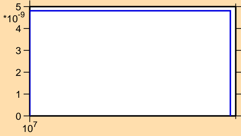
\sigma vs. E for ^{247}\text{Cf}(\text{mt117})
