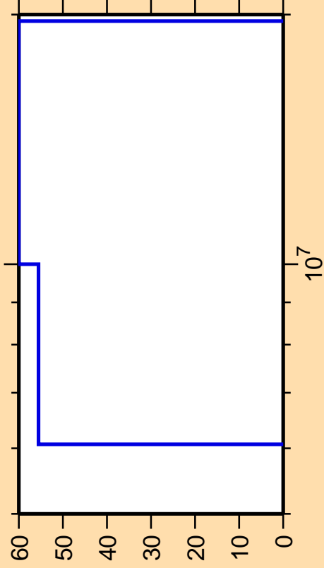
\Delta\sigma/\sigma vs. E for ^{247}\text{Cf}(n,2n)
