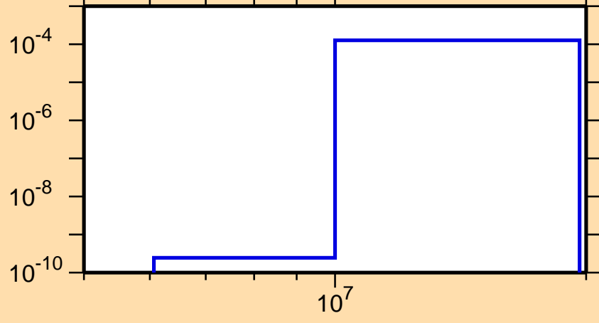
\sigma vs. E for ^{247}\text{Cf}(n,np)
