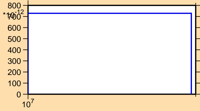
\sigma vs. E for ^{247}\text{Cf}(n,nt)
