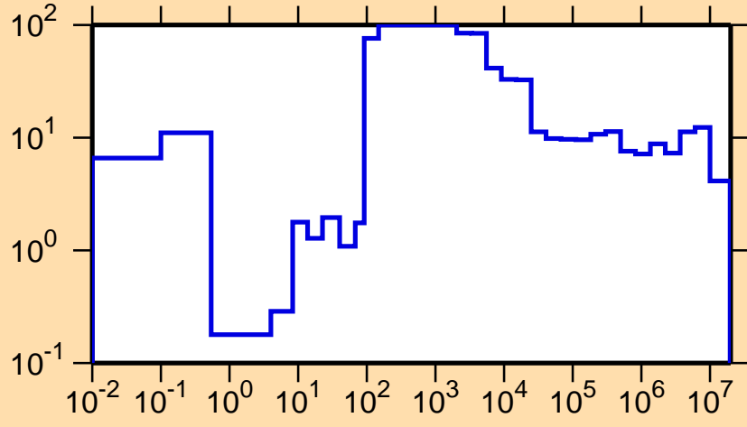
\Delta\sigma/\sigma vs. E for ^{247}\text{Cf}(n,el.)
