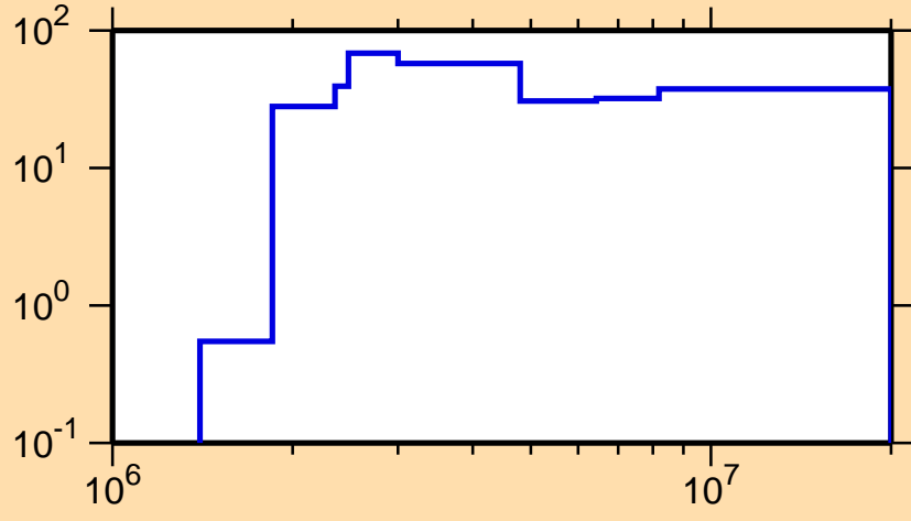
\Delta\sigma/\sigma vs. E for ^{247}\text{Cf}(n,p)
