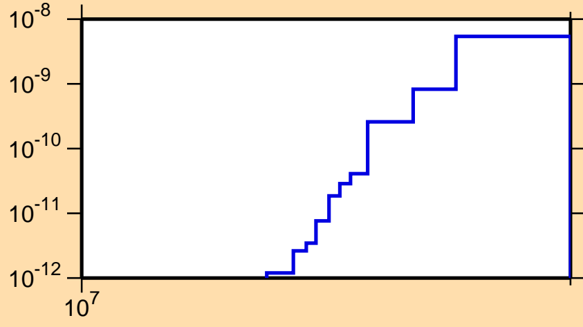
\sigma vs. E for ^{248}\text{Cf}(\text{mt } 45)
