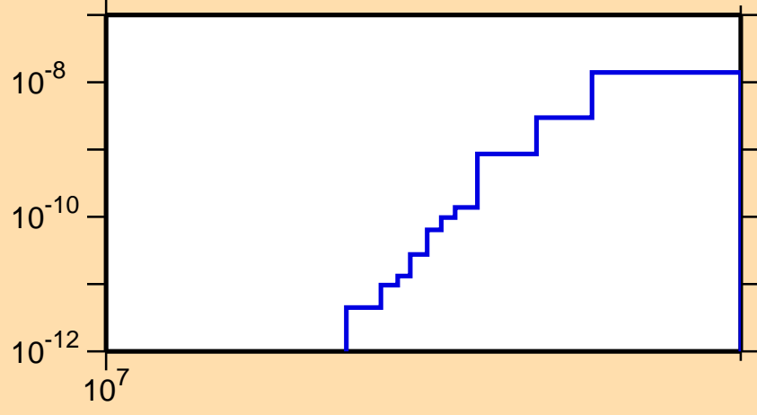
\sigma vs. E for ^{248}\text{Cf}(\text{mt117})
