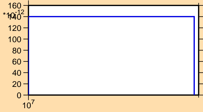
\sigma vs. E for ^{248}\text{Cf}(\text{mt } 45)
