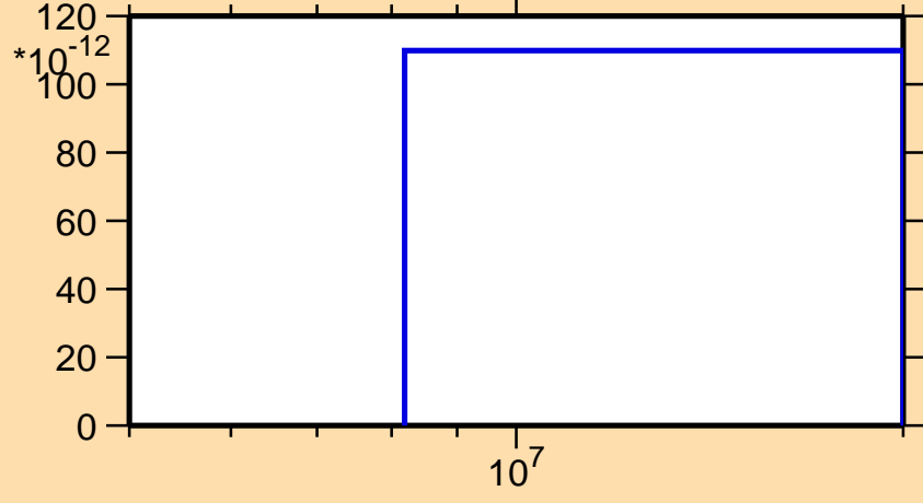
\sigma vs. E for ^{248}\text{Cf}(n,p\alpha)
