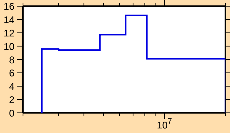
\Delta\sigma/\sigma vs. E for ^{249}\text{Cf}(n,n\text{cont.})
