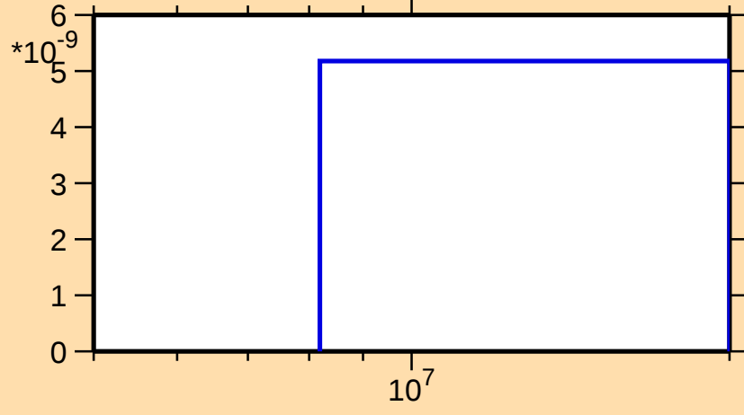
\sigma vs. E for ^{249}\text{Cf}(n,2np)
