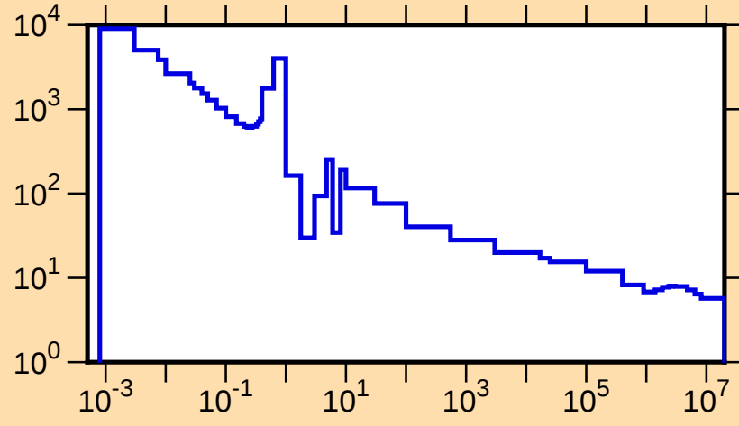
\sigma vs. E for ^{249}\text{Cf}(n,\text{tot.})
