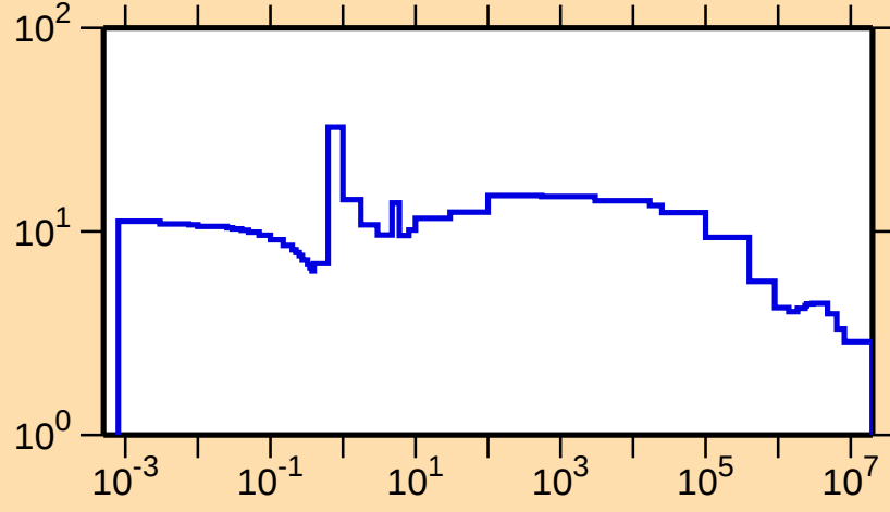
\sigma vs. E for ^{249}\text{Cf}(n,\text{el.})
