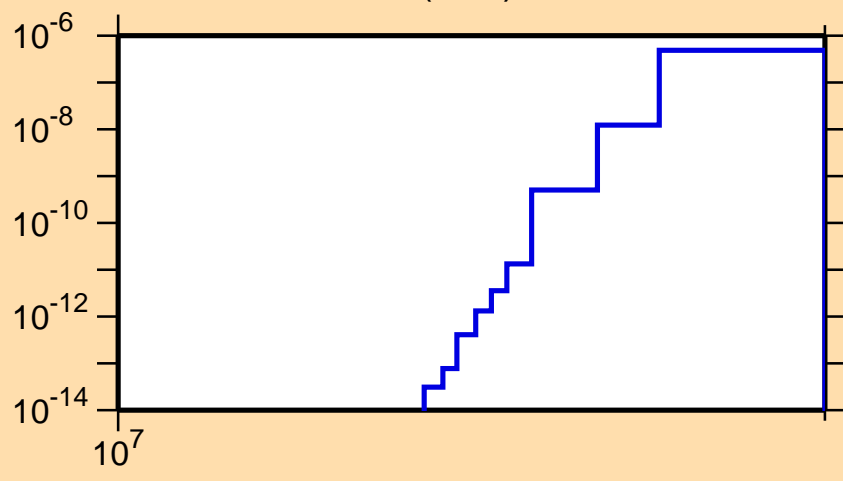
\sigma vs. E for ^{250}\text{Cf}(n,nt)
