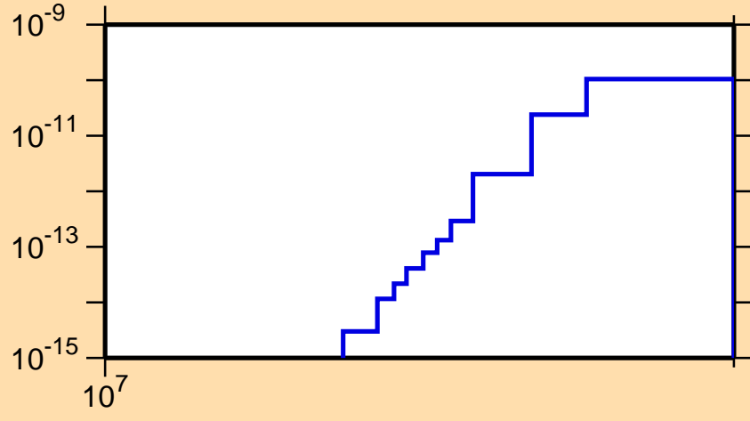
\sigma vs. E for ^{250}\text{Cf}(\text{mt117})
