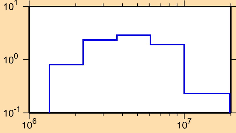
\sigma vs. E for ^{250}\text{Cf}(n,n\text{cont.})
