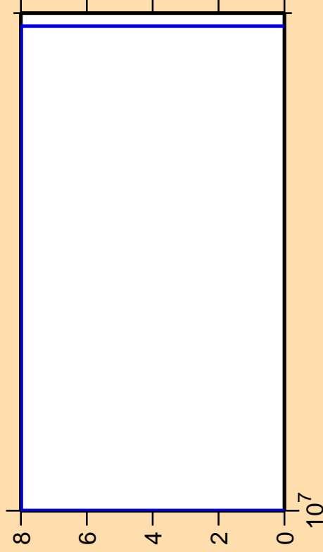
\Delta\sigma/\sigma vs. E for ^{250}\text{Cf}(\text{mt117})
