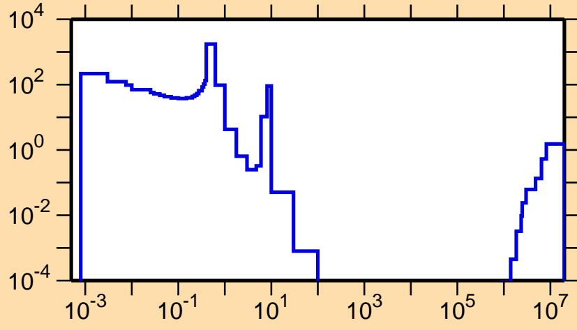
\sigma vs. E for ^{250}\text{Cf}(n,f)
