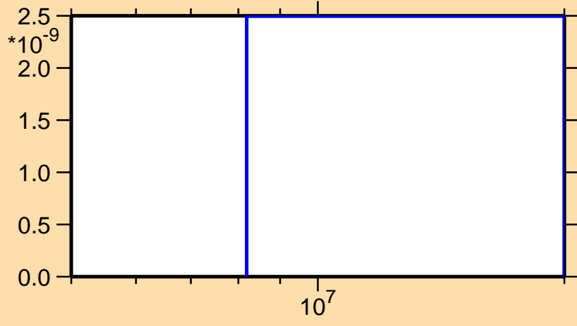
\sigma vs. E for ^{250}\text{Cf}(n,nd)
