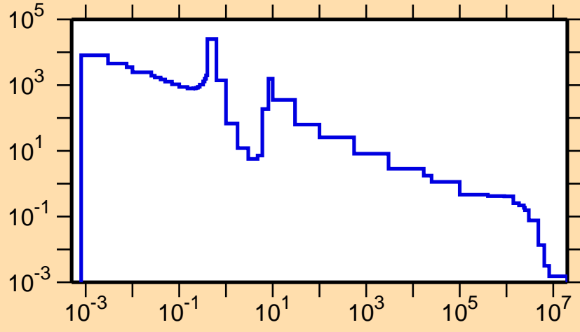
\sigma vs. E for ^{250}\text{Cf}(n,\gamma)
