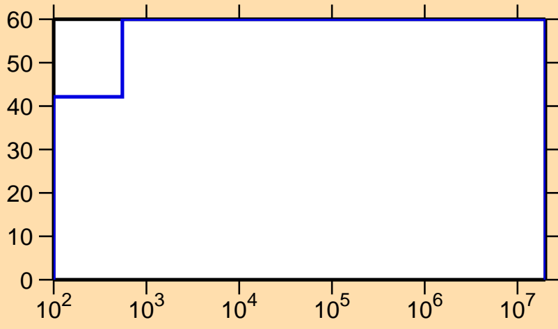
\Delta\sigma/\sigma vs. E for ^{250}\text{Cf}(n,\gamma)
