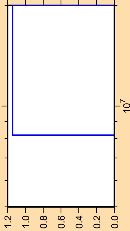
\Delta\sigma/\sigma vs. E for ^{250}\text{Cf}(n,p\alpha)
