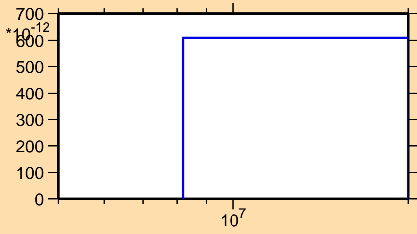
\sigma vs. E for ^{250}\text{Cf}(n,2np)
