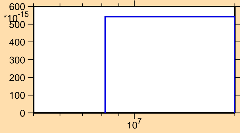
\sigma vs. E for ^{250}\text{Cf}(n,p\alpha)
