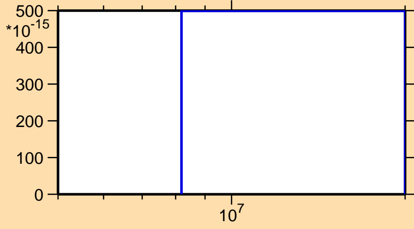
\sigma vs. E for ^{250}\text{Cf}(\text{mt } 45)
