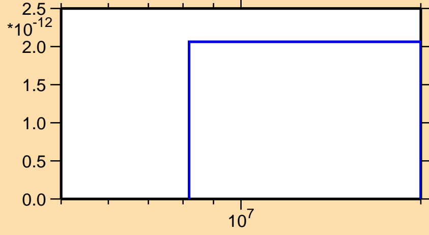
\sigma vs. E for ^{250}\text{Cf}(\text{mt117})
