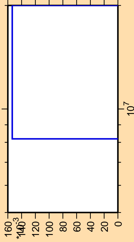
\Delta\sigma/\sigma vs. E for ^{250}\text{Cf}(n,\text{He3})
