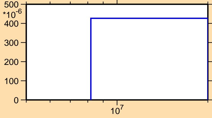
\sigma vs. E for ^{250}\text{Cf}(n,3n\alpha)
