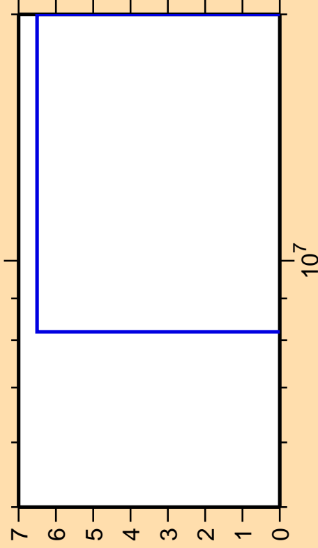
\Delta\sigma/\sigma vs. E for ^{250}\text{Cf}(\text{mt117})
