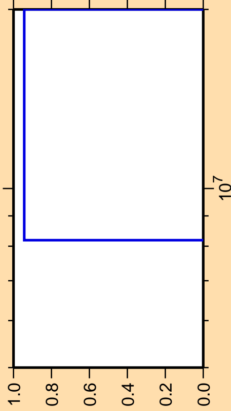
\Delta\sigma/\sigma vs. E for ^{250}\text{Cf}(\text{mt } 45)
