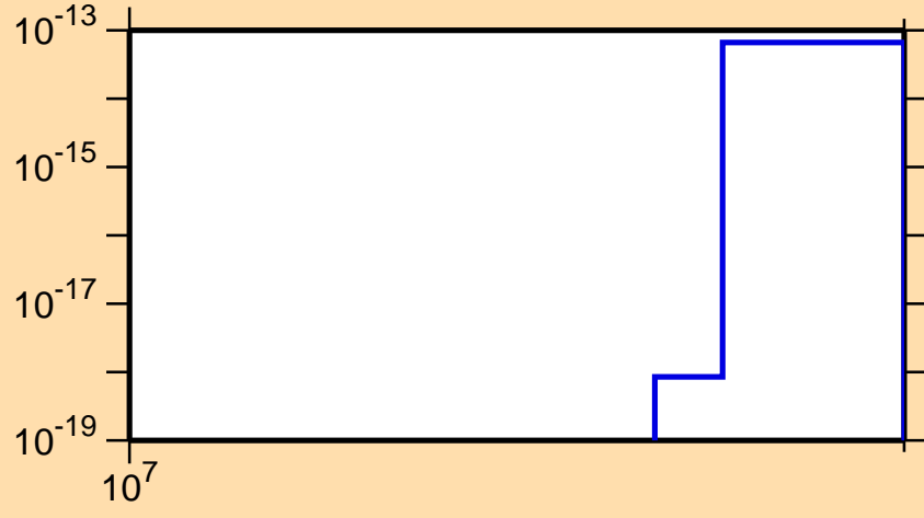
\sigma vs. E for ^{251}\text{Cf}(\text{mt 11})
