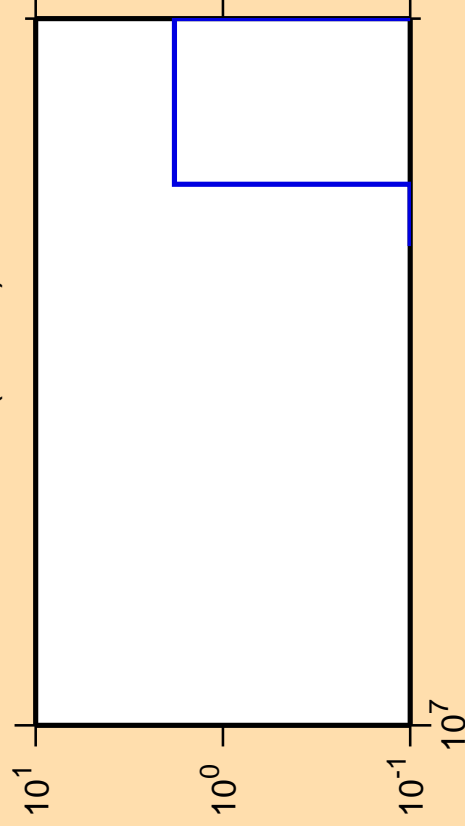
\Delta\sigma/\sigma vs. E for ^{251}\text{Cf}(\text{mt } 45)
