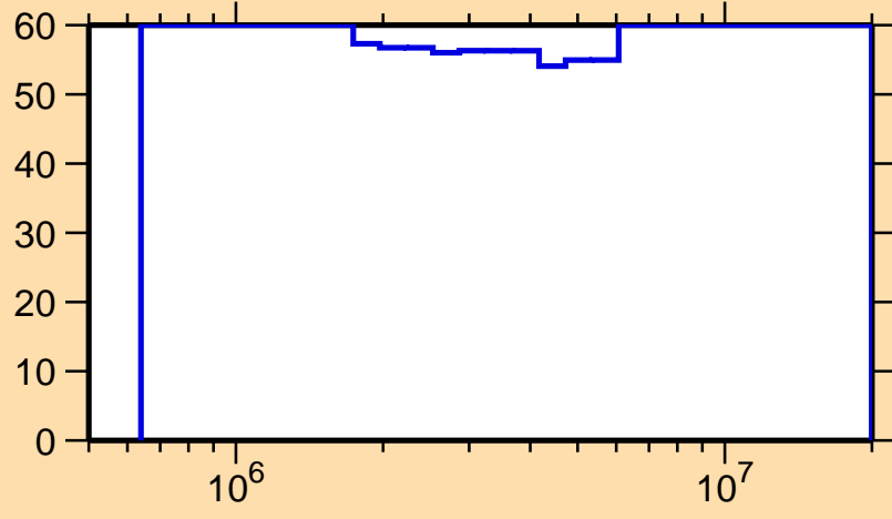
\Delta\sigma/\sigma vs. E for ^{251}\text{Cf}(n,ncont.)
