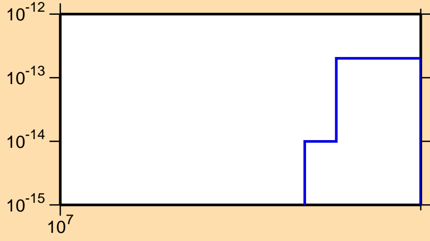
\sigma vs. E for ^{251}\text{Cf}(\text{mt } 45)
