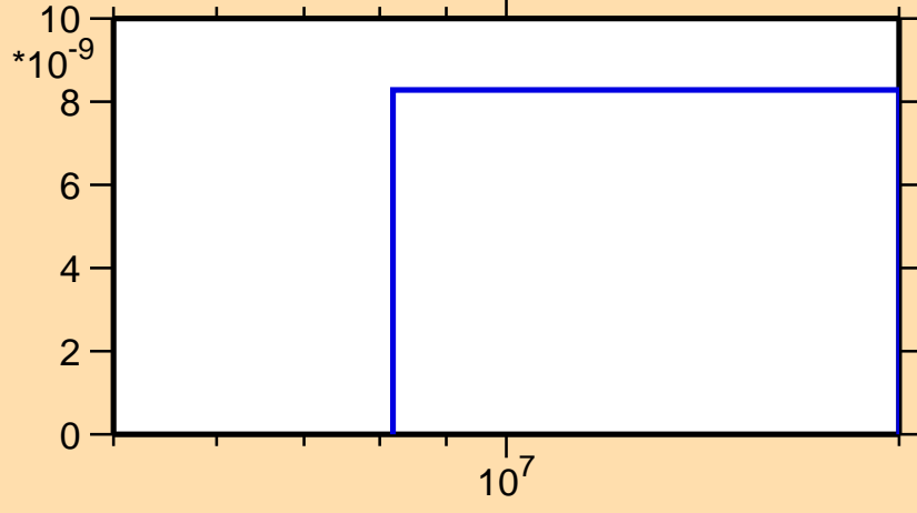
\sigma vs. E for ^{251}\text{Cf}(n,p\alpha)
