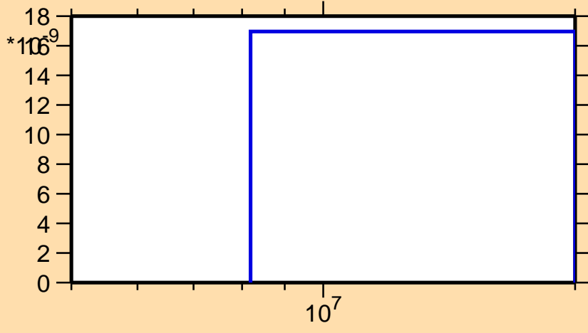
\sigma vs. E for ^{251}\text{Cf}(n,nt)
