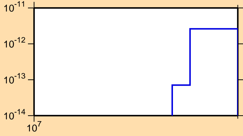
\sigma vs. E for ^{252}\text{Cf}(n,\text{He3})
