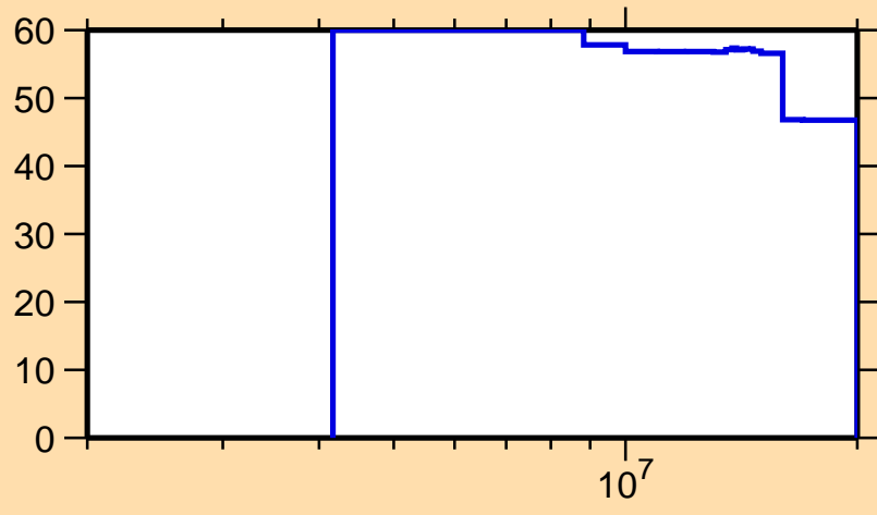
\Delta\sigma/\sigma vs. E for ^{252}\text{Cf}(n,f)
