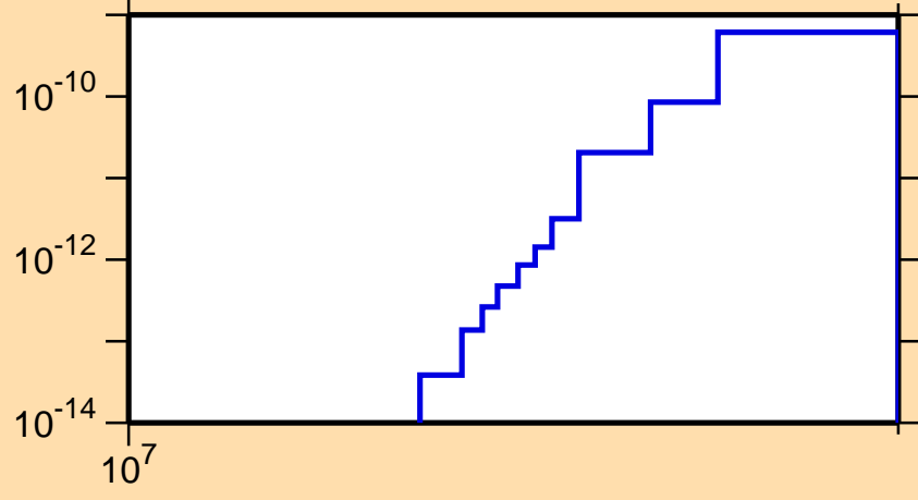
\sigma vs. E for ^{252}\text{Cf}(\text{mt117})
