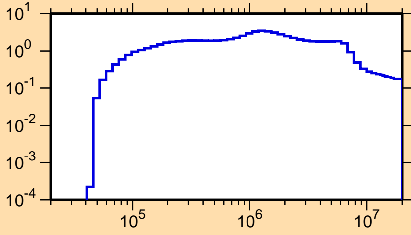
\sigma vs. E for ^{252}\text{Cf}(n,\text{inel.})
