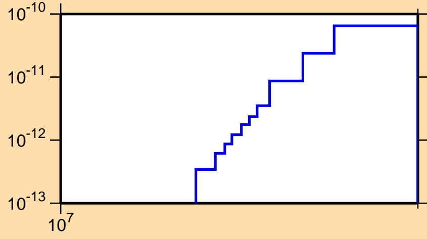
\sigma vs. E for ^{252}\text{Cf}(n,p\alpha)
