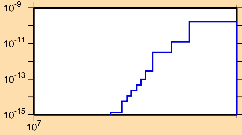
\sigma vs. E for ^{252}\text{Cf}(\text{mt } 45)
