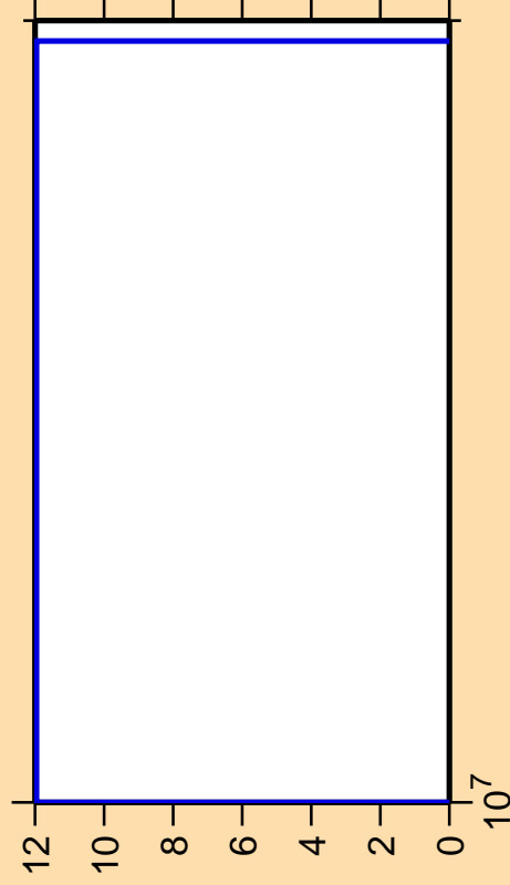
\Delta\sigma/\sigma vs. E for ^{252}\text{Cf} (mt 45)
