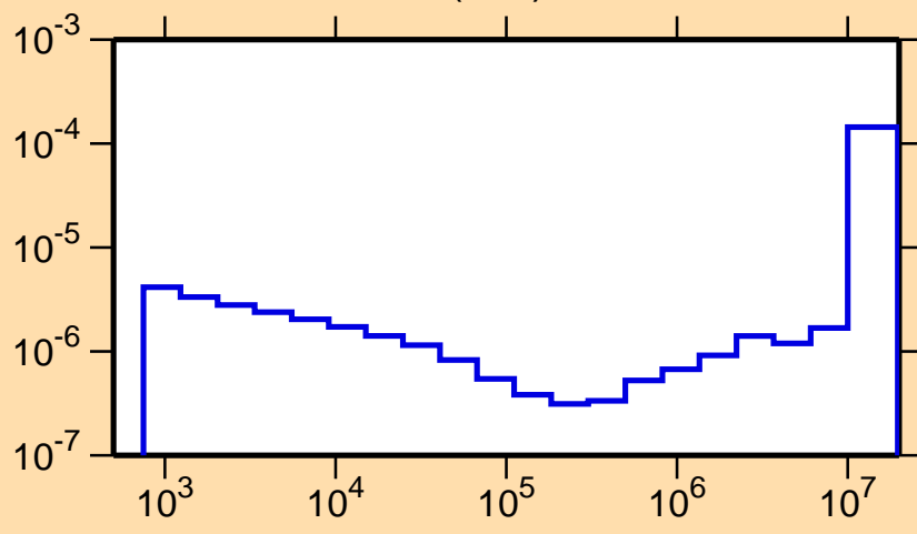
\sigma vs. E for ^{252}\text{Cf}(n,\alpha)
