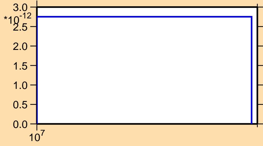
\sigma vs. E for ^{252}\text{Cf} (mt 45)
