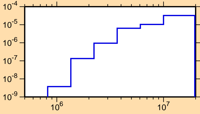
\sigma vs. E for ^{252}\text{Cf}(n,n\alpha)
