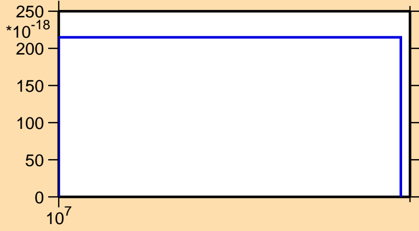
\sigma vs. E for ^{252}\text{Cf} (mt 11)
