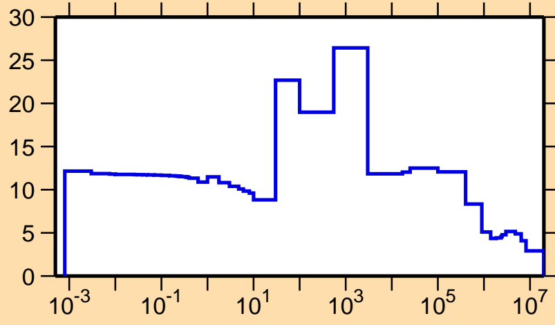
\sigma vs. E for ^{252}\text{Cf}(n,\text{el.})
