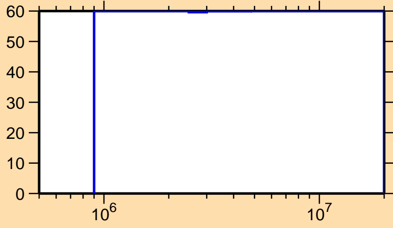
\Delta\sigma/\sigma vs. E for ^{252}\text{Cf}(n,n\text{cont.})
