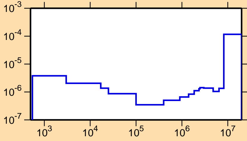
\sigma vs. E for ^{252}\text{Cf}(n,\alpha)
