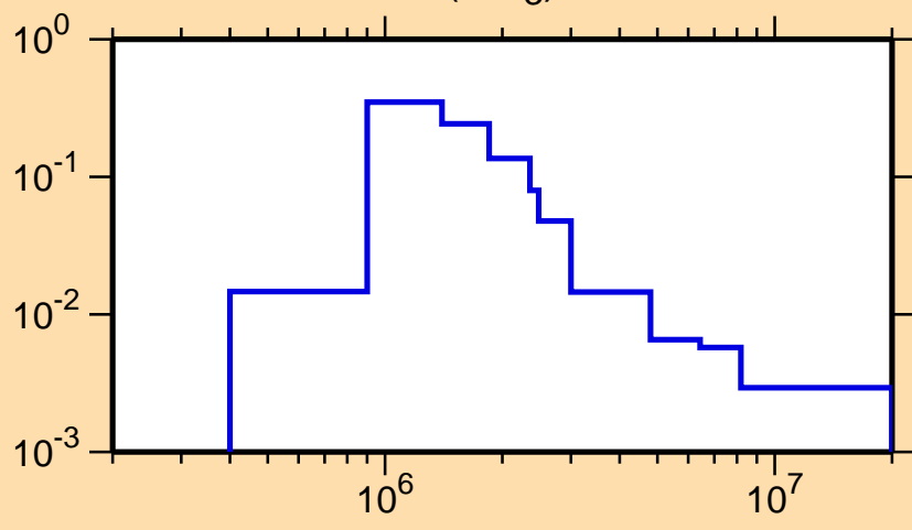
\sigma vs. E for ^{252}\text{Cf}(n,n_3)
