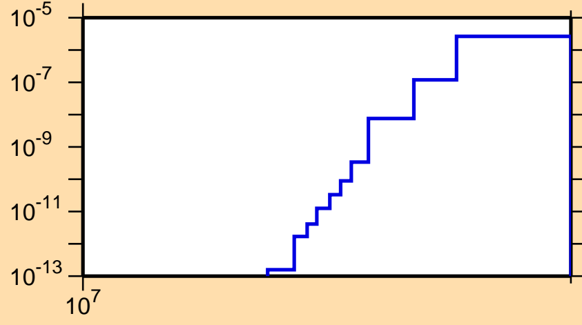
\sigma vs. E for ^{253}\text{Cf}(n,nt)
