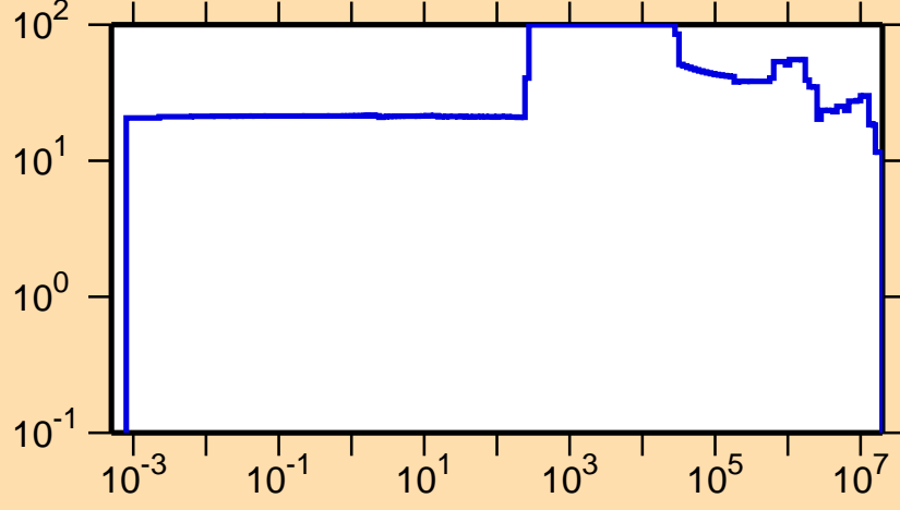
\Delta\sigma/\sigma vs. E for ^{253}\text{Cf}(n,el.)
