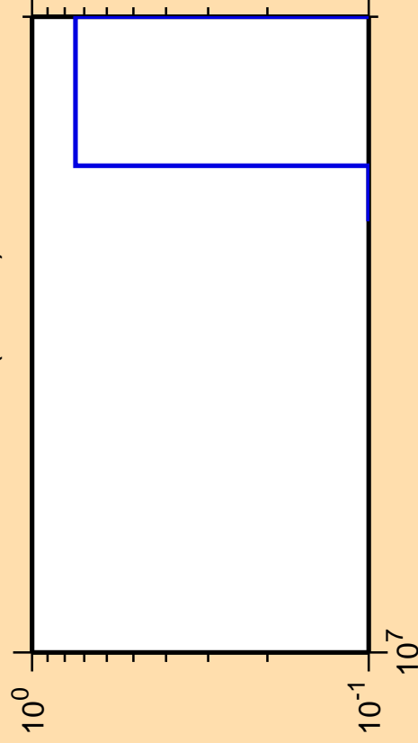
\Delta\sigma/\sigma vs. E for ^{253}\text{Cf} (mt 11)
