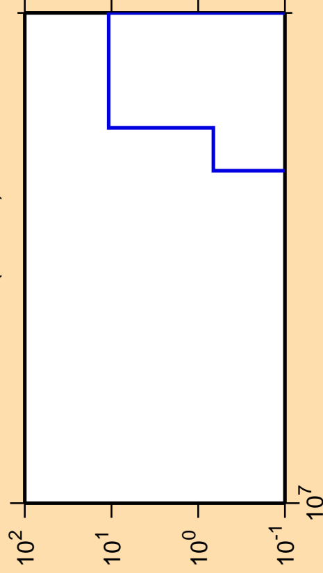
\Delta\sigma/\sigma vs. E for ^{253}\text{Cf}(\text{mt } 45)
