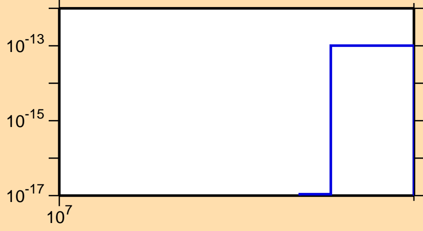
\sigma vs. E for ^{253}\text{Cf} (mt 11)
