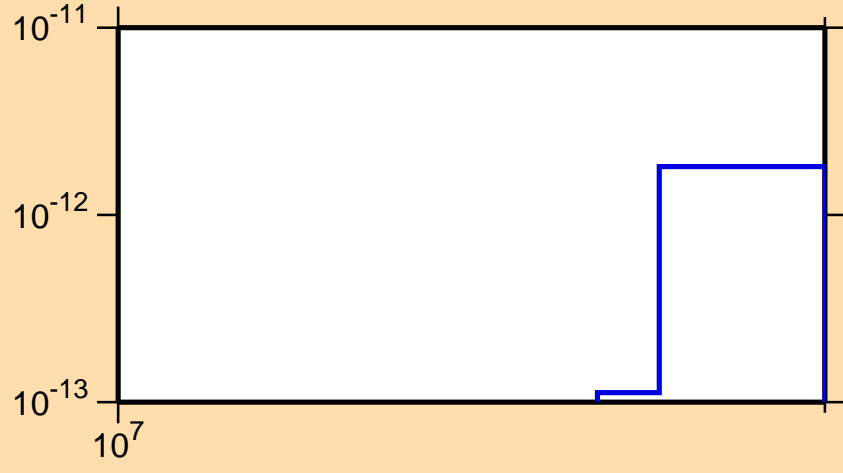
\sigma vs. E for ^{253}\text{Cf}(\text{mt } 45)
