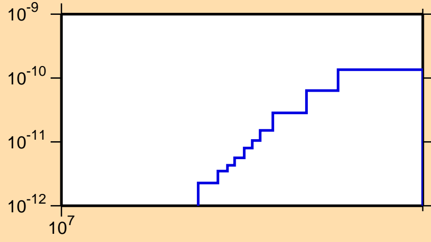
\sigma vs. E for ^{253}\text{Cf}(n,p\alpha)
