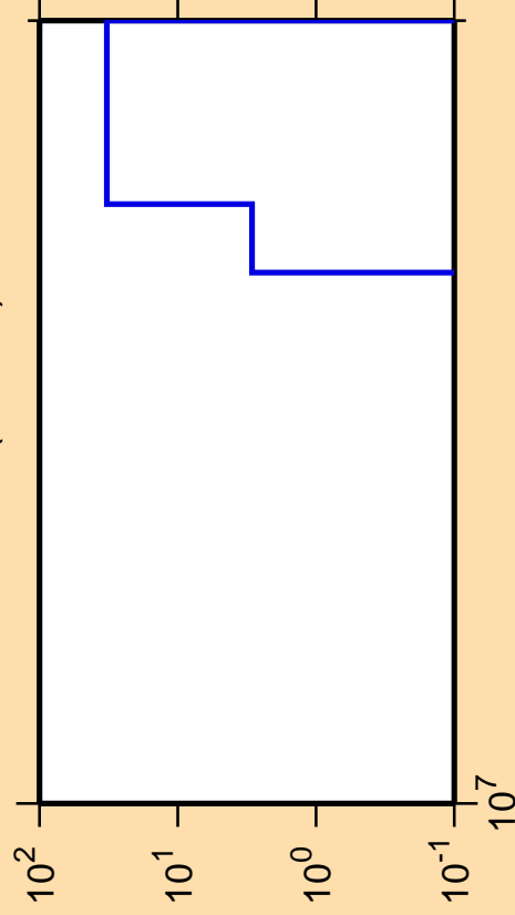
\Delta\sigma/\sigma vs. E for ^{253}\text{Cf}(\text{mt117})
