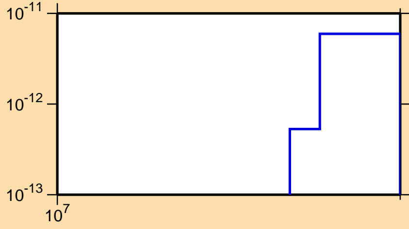
\sigma vs. E for ^{253}\text{Cf}(\text{mt117})
