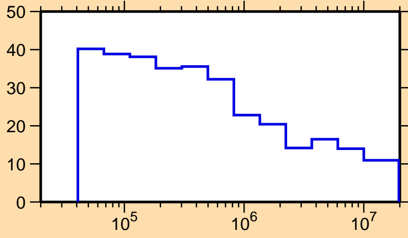
\Delta\sigma/\sigma vs. E for ^{253}\text{Cf}(n,\text{tot.})
