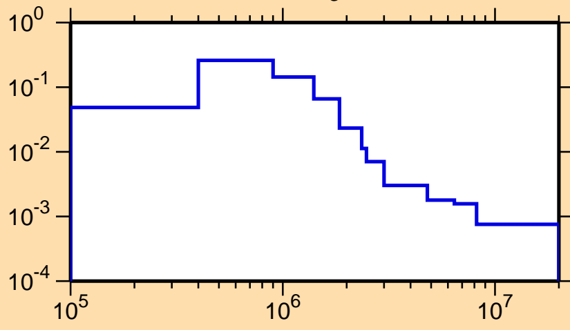
\sigma vs. E for ^{253}\text{Cf}(n,n_3)
