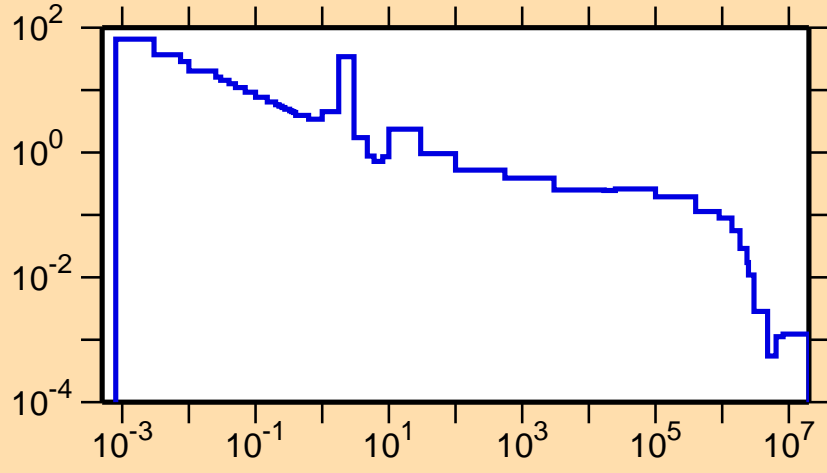
\sigma vs. E for ^{253}\text{Cf}(n,\gamma)
