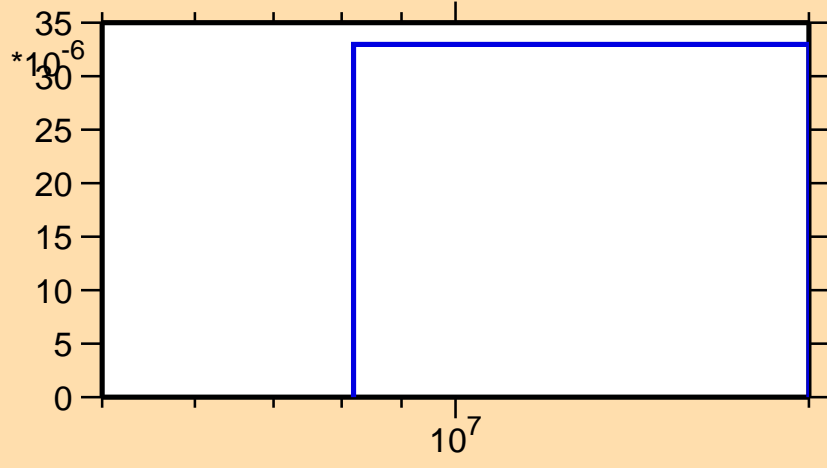
\sigma vs. E for ^{253}\text{Cf}(n,d)
