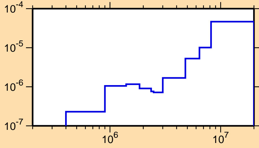
\sigma vs. E for ^{253}\text{Cf}(n,n\alpha)
