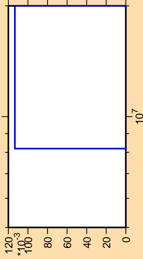
\Delta\sigma/\sigma vs. E for ^{253}\text{Cf}(\text{mt } 45)
