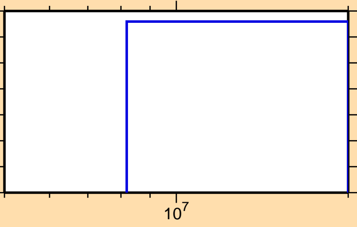
\sigma vs. E for ^{253}\text{Cf}(n,d)
