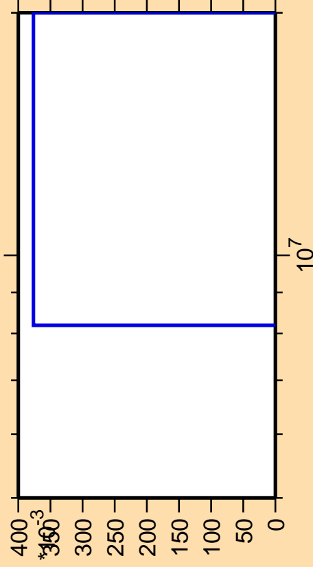
\Delta\sigma/\sigma vs. E for ^{253}\text{Cf}(\text{mt117})
