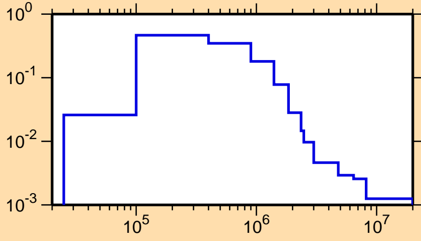
\sigma vs. E for ^{253}\text{Cf}(n,n_1)
