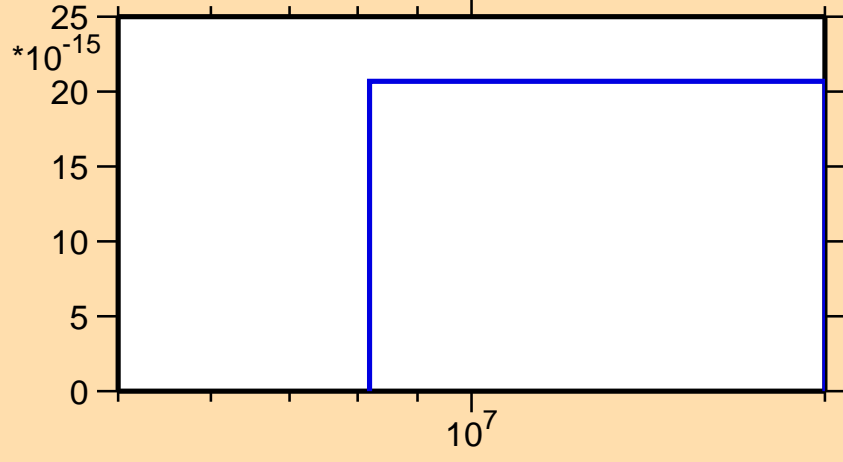
\sigma vs. E for ^{253}\text{Cf}(\text{mt } 45)
