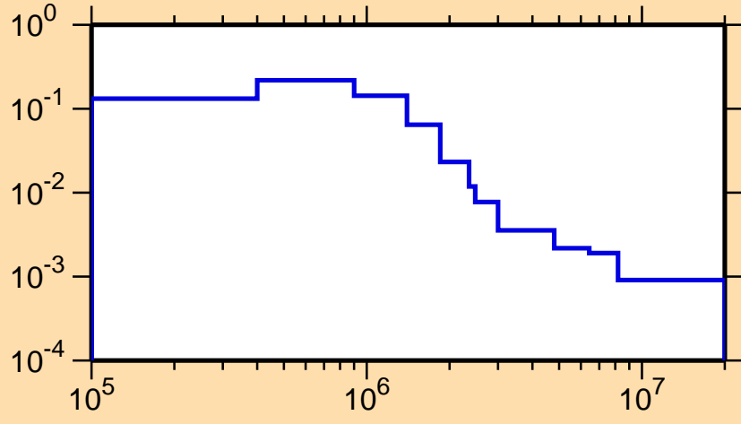
\sigma vs. E for ^{253}\text{Cf}(n,n_2)
