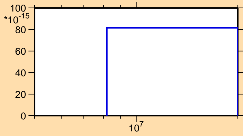
\sigma vs. E for ^{253}\text{Cf}(\text{mt117})
