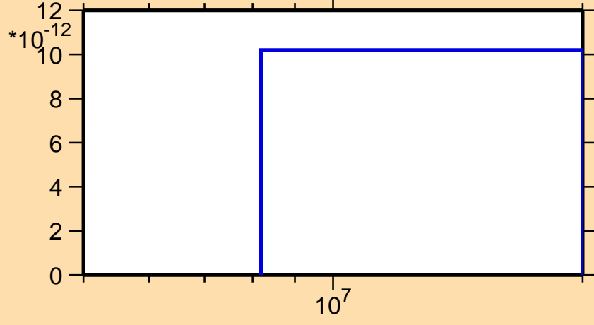
\sigma vs. E for ^{253}\text{Cf}(n,p\alpha)
