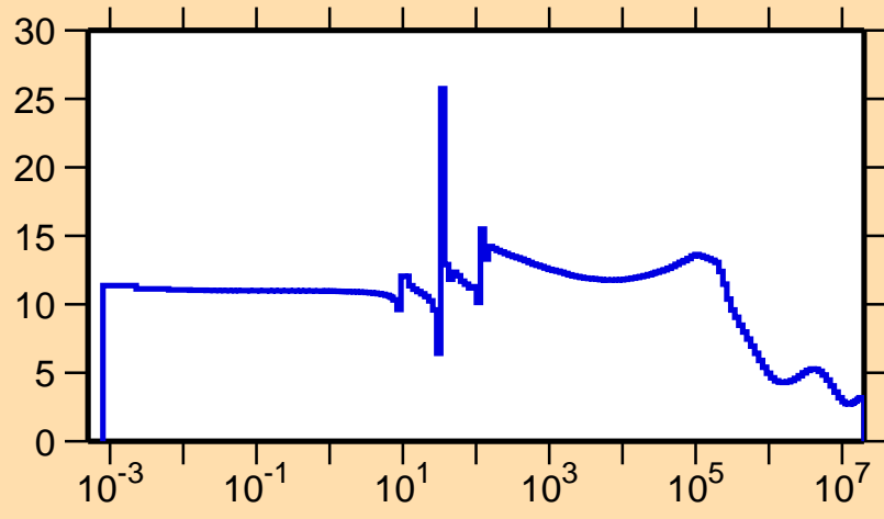
\sigma vs. E for ^{254}\text{Cf}(n,\text{el.})
