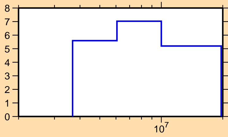
\Delta\sigma/\sigma vs. E for ^{254}\text{Cf}(n,\text{nonel.})
