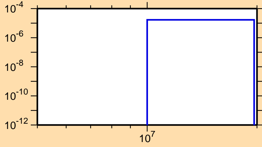
\sigma vs. E for ^{254}\text{Cf}(n,t)
