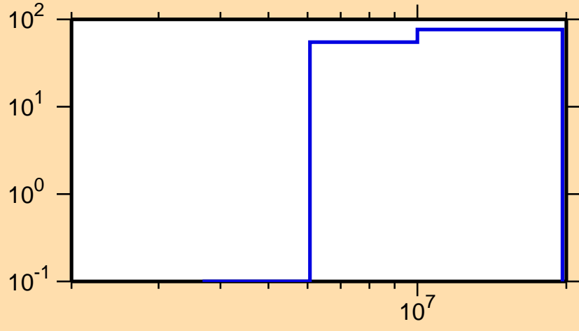
\Delta\sigma/\sigma vs. E for ^{254}\text{Cf}(n,p)
