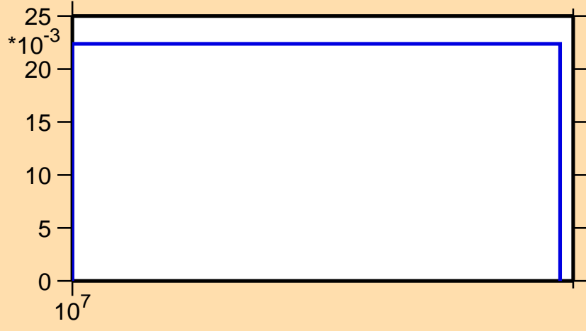
\sigma vs. E for ^{254}\text{Cf}(n,3n\alpha)
