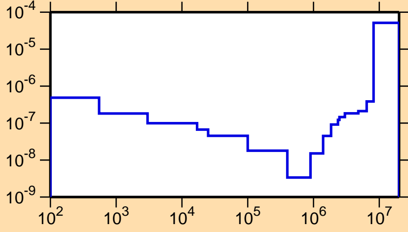
\sigma vs. E for ^{254}\text{Cf}(n,\alpha)
