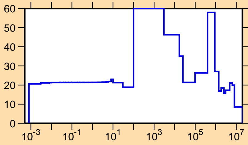
\Delta\sigma/\sigma vs. E for ^{254}\text{Cf}(n,el.)
