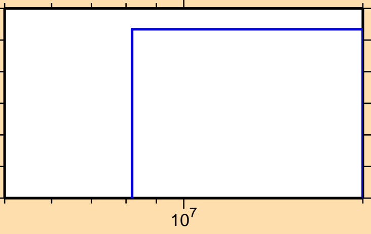
\sigma vs. E for ^{254}\text{Cf}(n,3n)
