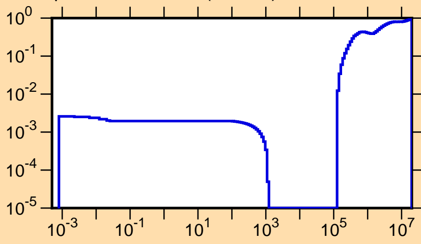
\mu vs. E for ^{255}\text{Cf}(\text{mt251})
