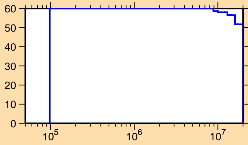
\Delta\sigma/\sigma vs. E for ^{255}\text{Cf}(n,n_1)
