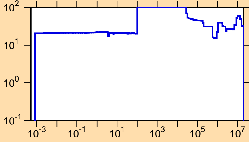
\Delta\sigma/\sigma vs. E for ^{255}\text{Cf}(n,el.)
