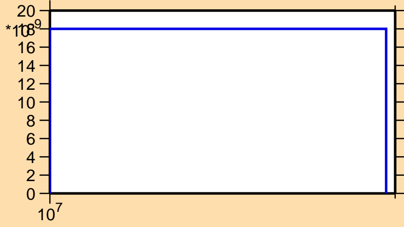
\sigma vs. E for ^{255}\text{Cf}(n,nt)
