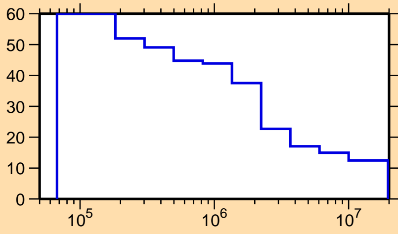
\Delta\sigma/\sigma vs. E for ^{255}\text{Cf}(n,\text{nonel.})
