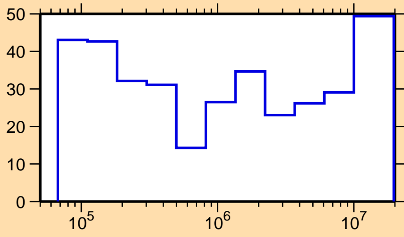
\Delta\sigma/\sigma vs. E for ^{255}\text{Cf}(n,\text{el.})
