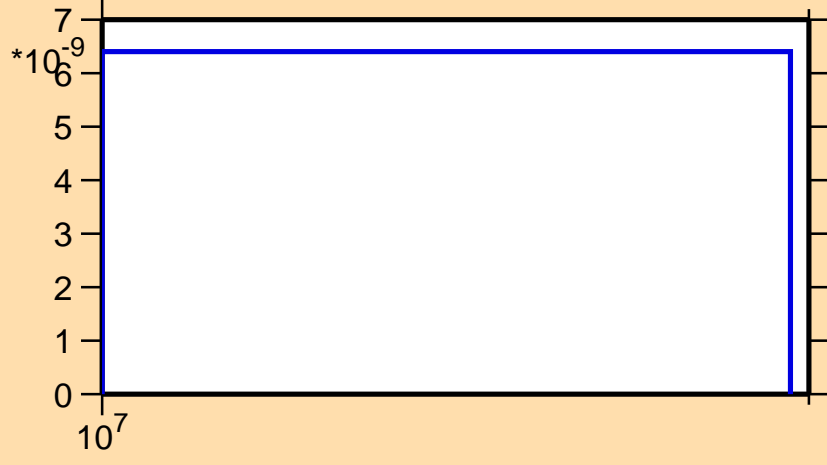
\sigma vs. E for ^{255}\text{Cf}(n,nd)
