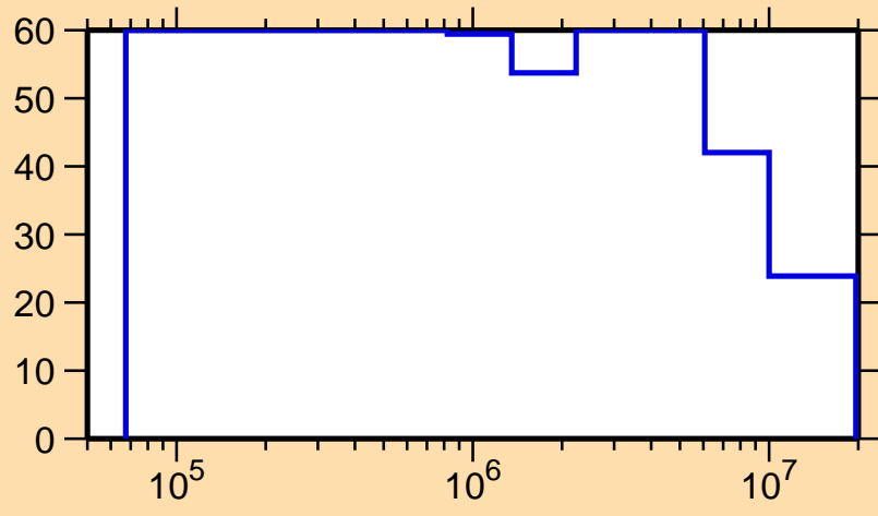
\Delta\sigma/\sigma vs. E for ^{255}\text{Cf}(n,f)
