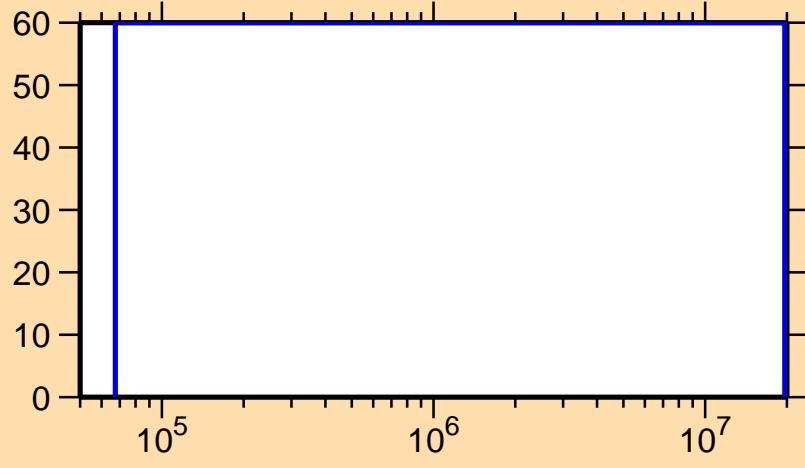
\Delta\sigma/\sigma vs. E for ^{255}\text{Cf}(n,n\text{cont.})
