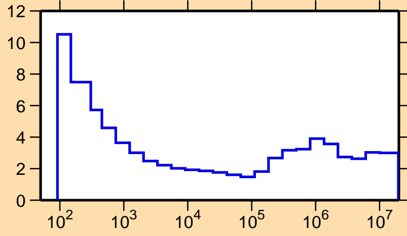
\sigma vs. E for ^{255}\text{Cf}(n,\text{nonel.})
