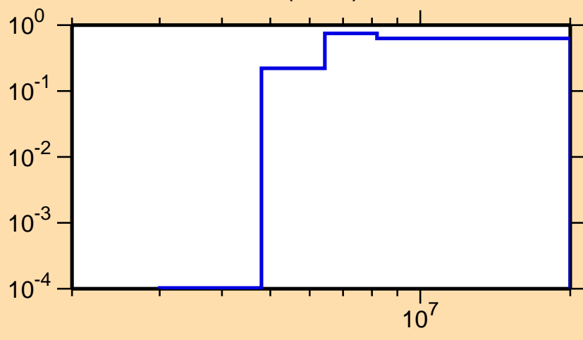
\sigma vs. E for ^{255}\text{Cf}(n,2n)
