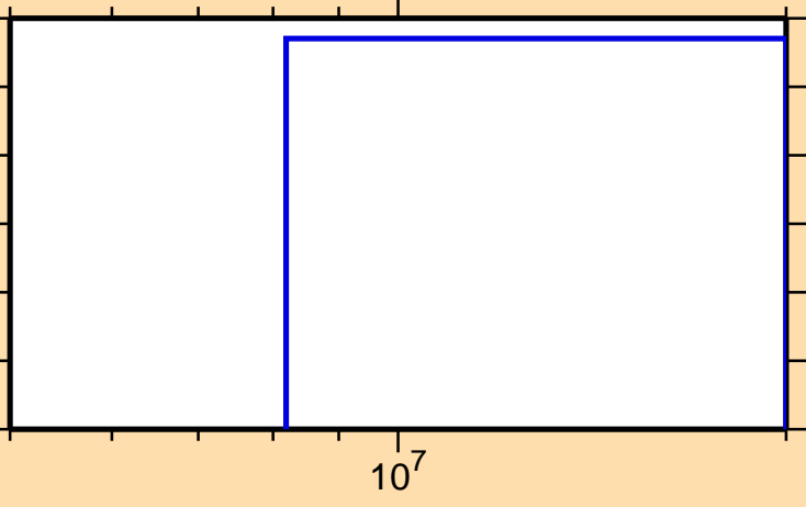
\sigma vs. E for ^{255}\text{Cf}(n,nd)
