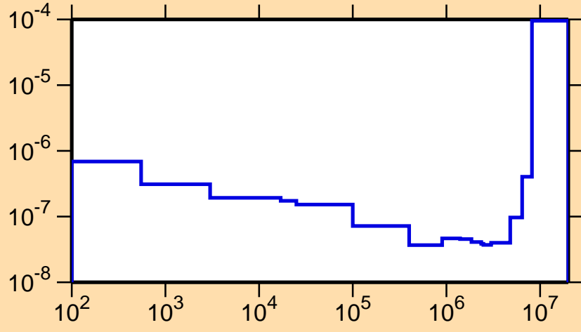
\sigma vs. E for ^{255}\text{Cf}(n,\alpha)
