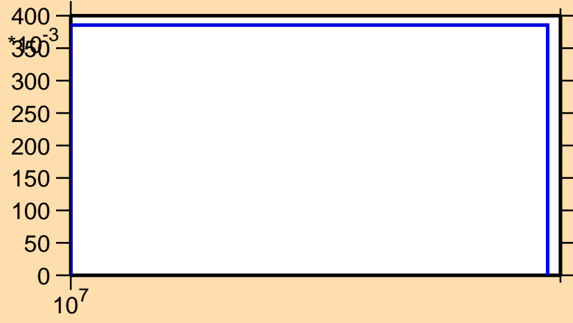
\sigma vs. E for ^{256}\text{Cf}(n,3n)
