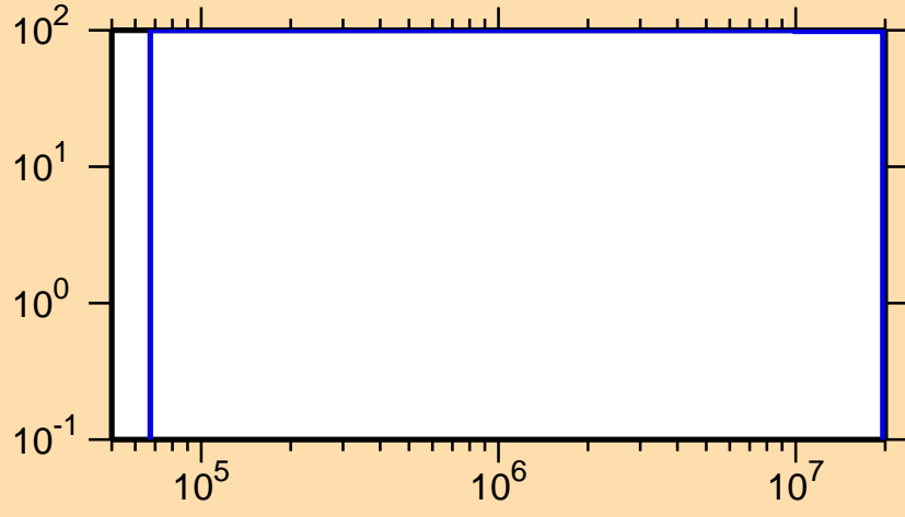
\Delta\sigma/\sigma vs. E for ^{256}\text{Cf}(n,n\text{cont.})
