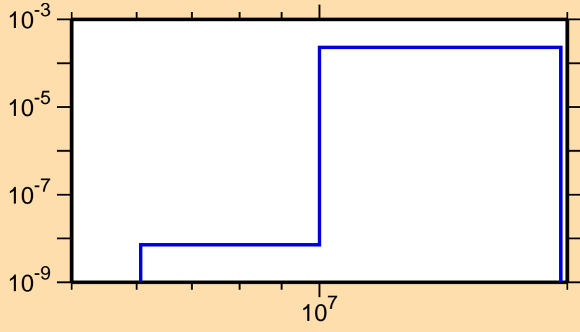
\sigma vs. E for ^{256}\text{Cf}(n,p)
