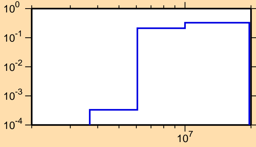
\sigma vs. E for ^{256}\text{Cf}(n,2n)
