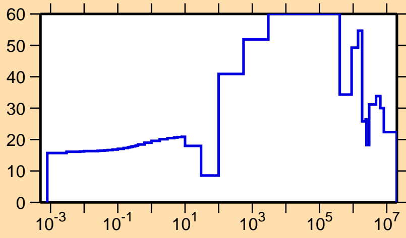
\Delta\sigma/\sigma vs. E for ^{256}\text{Cf}(n,\text{el.})
