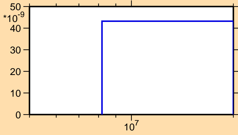
\sigma vs. E for ^{256}\text{Cf}(n,3n\alpha)
