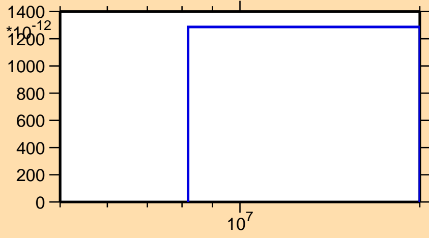
\sigma vs. E for ^{256}\text{Cf}(n,nd)
