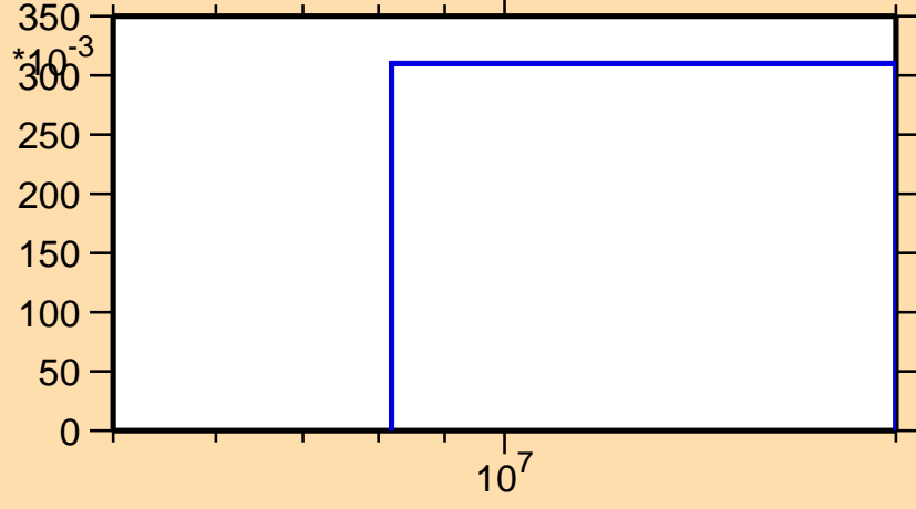
\sigma vs. E for ^{256}\text{Cf}(n,3n)
