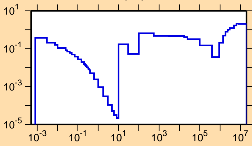
\sigma vs. E for ^{256}\text{Cf}(n,f)
