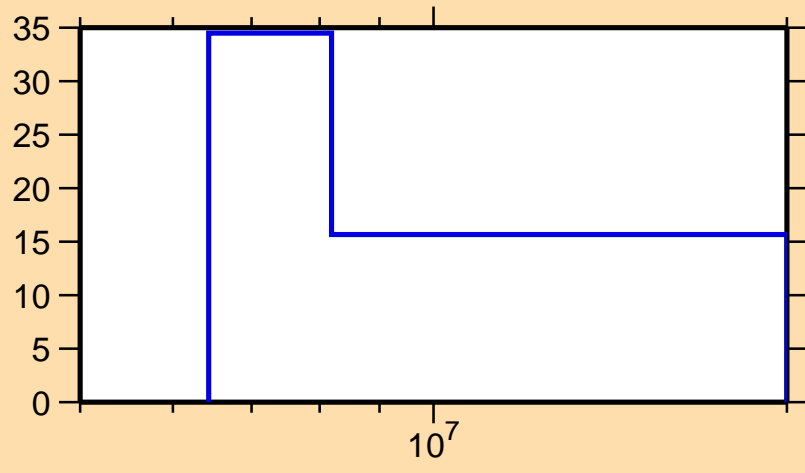
\Delta\sigma/\sigma vs. E for ^{256}\text{Cf}(n,\text{tot.})
