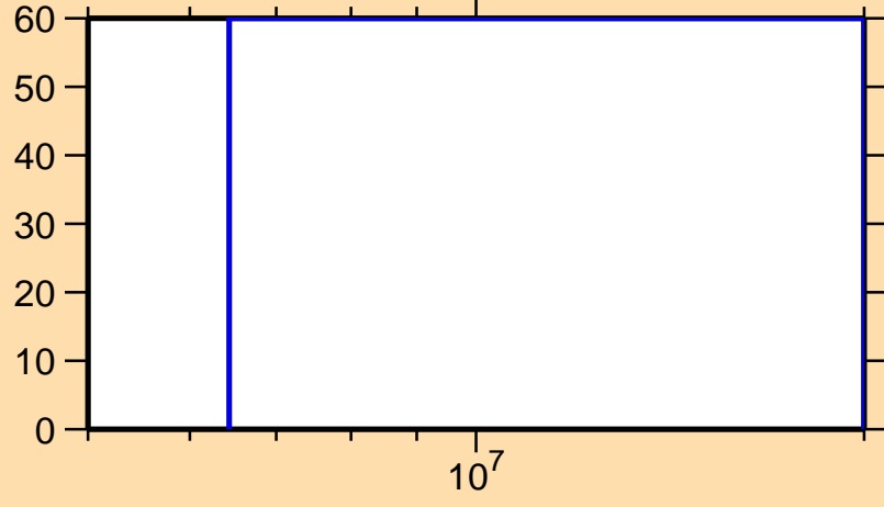
\Delta\sigma/\sigma vs. E for ^{256}\text{Cf}(n,p)
