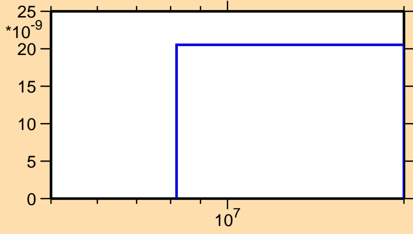
\sigma vs. E for ^{256}\text{Cf}(n,nt)
