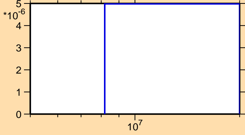
\sigma vs. E for ^{256}\text{Cf}(n,np)
