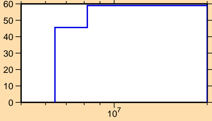
\Delta\sigma/\sigma vs. E for ^{256}\text{Cf}(n,\text{inel.})
