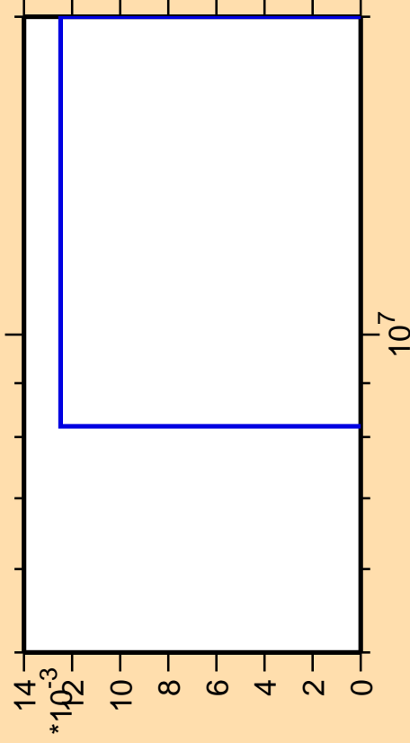
\Delta\sigma/\sigma vs. E for ^{256}\text{Cf}(n,\text{He3})
