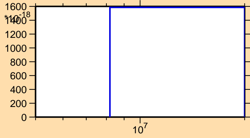
\sigma vs. E for ^{256}\text{Cf}(n,\text{He3})
