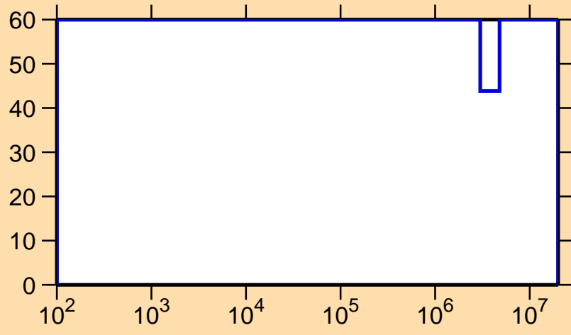
\Delta\sigma/\sigma vs. E for ^{256}\text{Cf}(n,\gamma)
