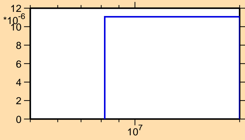
\sigma vs. E for ^{256}\text{Cf}(n,d)
