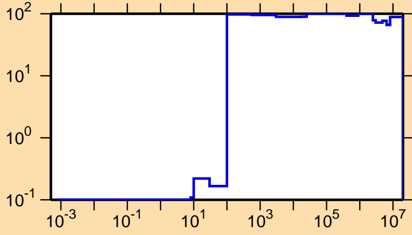
\Delta\sigma/\sigma vs. E for ^{256}\text{Cf}(n,f)
