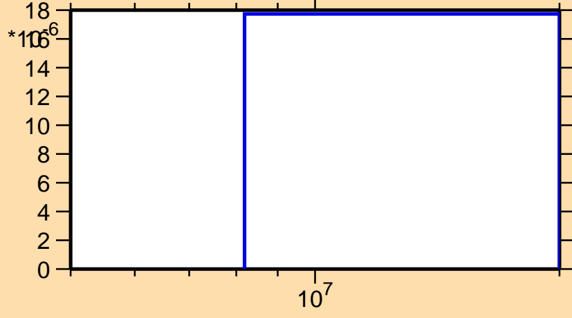
\sigma vs. E for ^{256}\text{Cf}(n,t)
