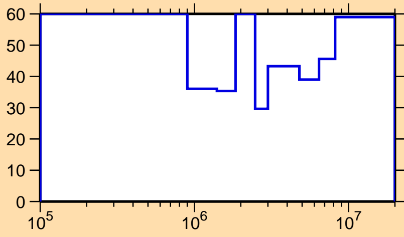
\Delta\sigma/\sigma vs. E for ^{256}\text{Cf}(n,\text{inel.})
