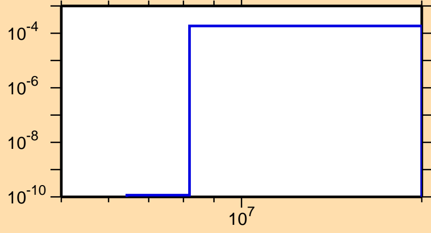
\sigma vs. E for ^{256}\text{Cf}(n,p)
