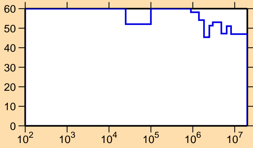
\Delta\sigma/\sigma vs. E for ^{256}\text{Cf}(n,\text{nonel.})
