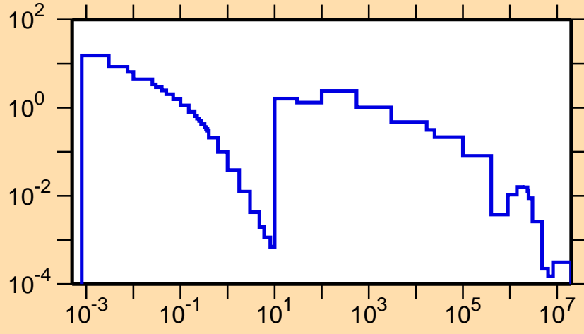
\sigma vs. E for ^{256}\text{Cf}(n,\gamma)
