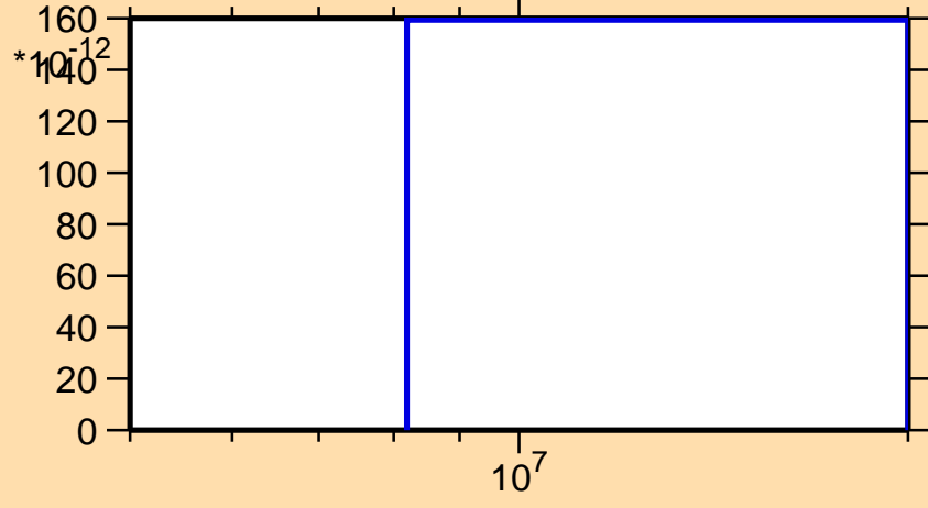
\sigma vs. E for ^{256}\text{Cf}(n,2np)
