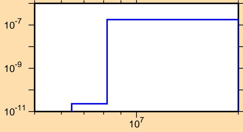
\sigma vs. E for ^{256}\text{Cf}(n,2n\alpha)
