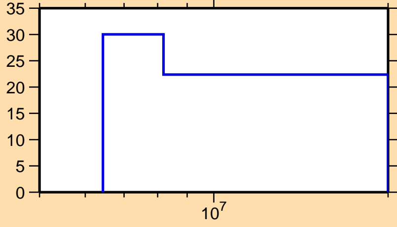
\Delta\sigma/\sigma vs. E for ^{256}\text{Cf}(n,el.)
