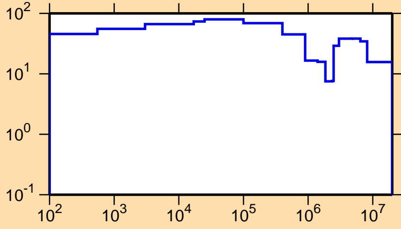
\Delta\sigma/\sigma vs. E for ^{256}\text{Cf}(n,\text{tot.})
