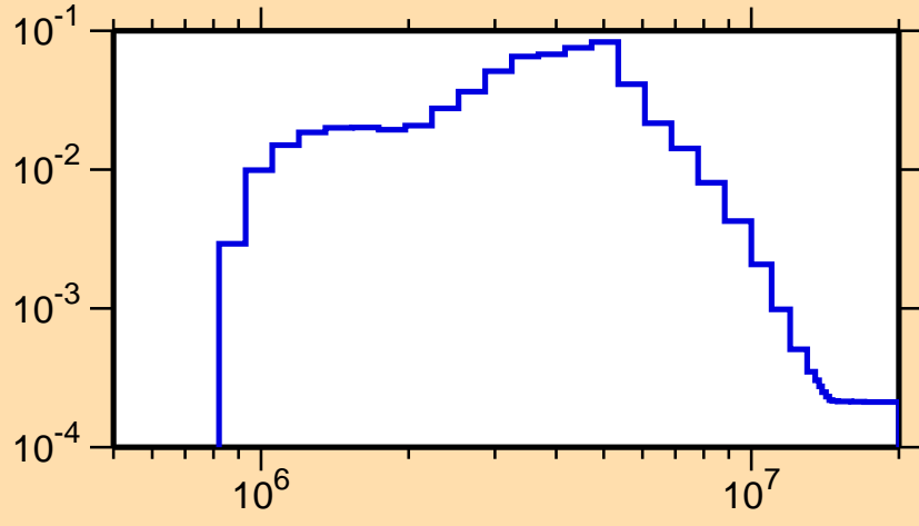
\sigma vs. E for ^{33}\text{Cl}(n,\text{inel.})
