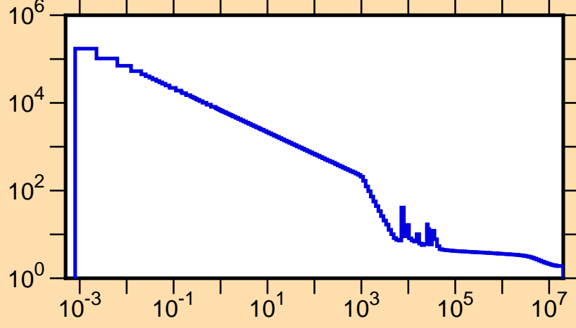
\sigma vs. E for ^{33}\text{Cl}(n,\text{tot.})
