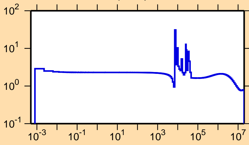
\sigma vs. E for ^{33}\text{Cl}(n,\text{el.})
