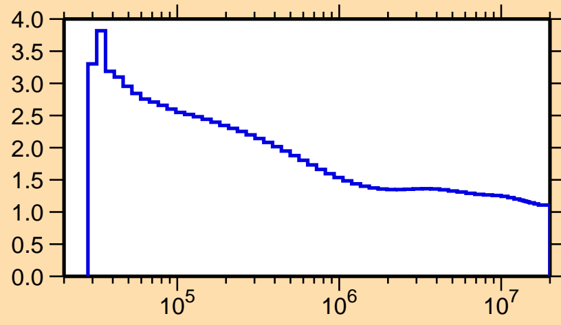
\sigma vs. E for ^{33}\text{Cl}(n,\text{nonel.})
