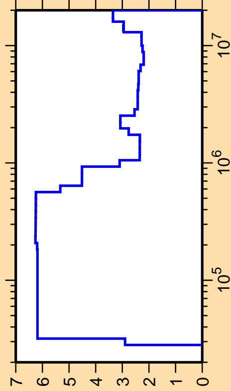
\Delta\sigma/\sigma vs. E for ^{33}\text{Cl}(n,\text{nonel.})
