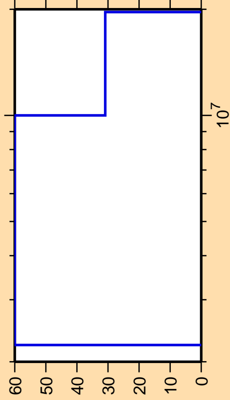
\Delta\sigma/\sigma vs. E for ^{33}\text{Cl}(n,\text{ncont.})
