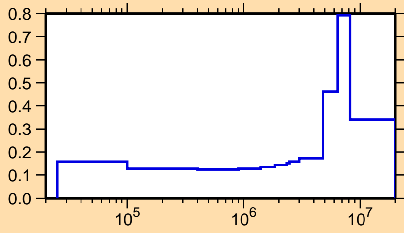
\sigma vs. E for ^{33}\text{Cl}(n,\alpha)
