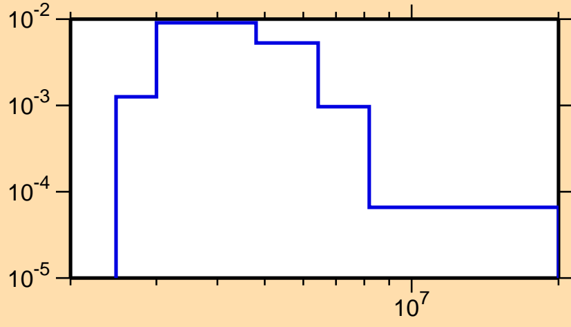
\sigma vs. E for ^{33}\text{Cl}(n,n_4)
