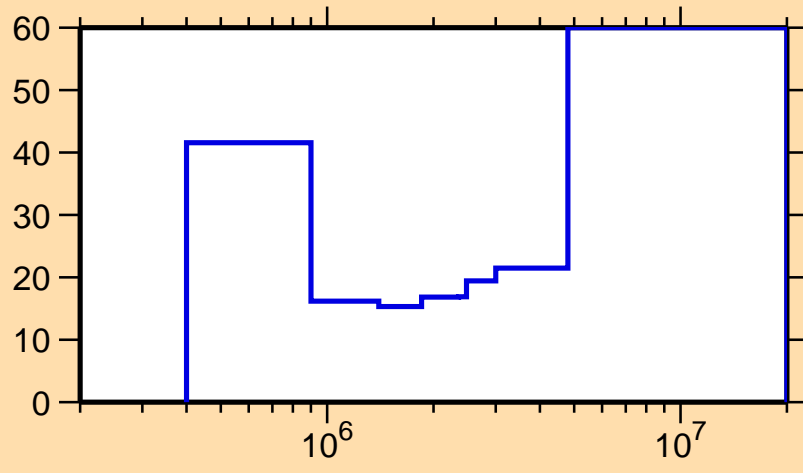
\Delta\sigma/\sigma vs. E for ^{33}\text{Cl}(n,n_1)
