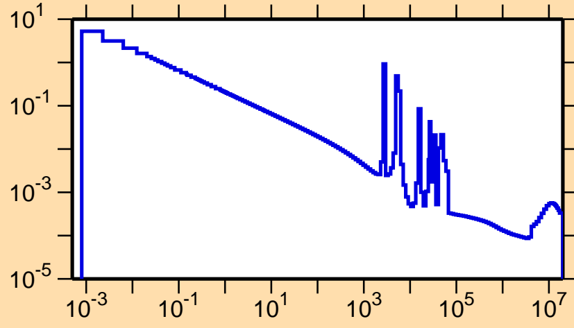
\sigma vs. E for ^{34}\text{Cl}(n,\gamma)
