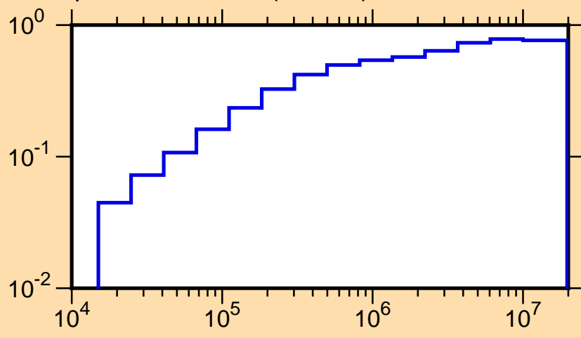
\mu vs. E for ^{34}\text{Cl}(\text{mt251})
