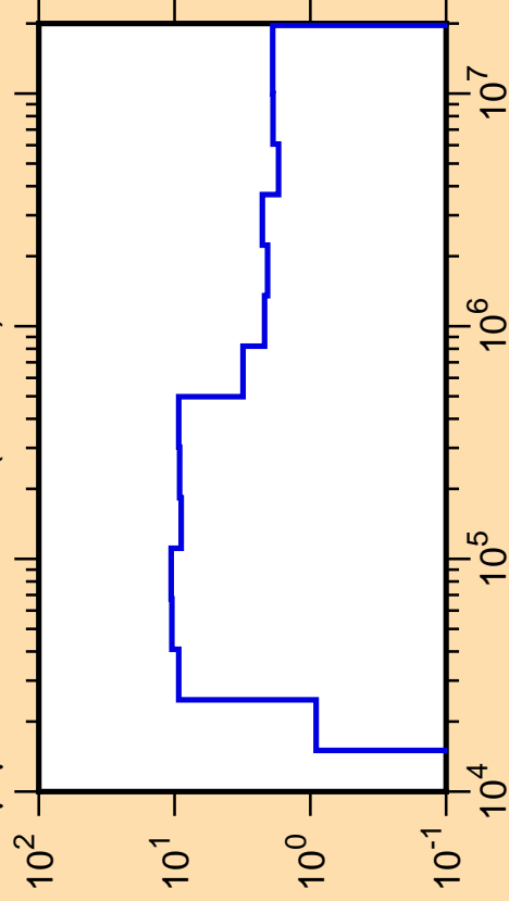
\Delta\mu/\mu vs. E for ^{34}\text{Cl}(\text{mt251})
