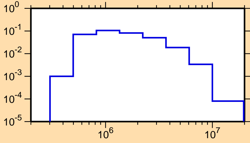
\sigma vs. E for ^{34}\text{Cl}(n,n_2)
