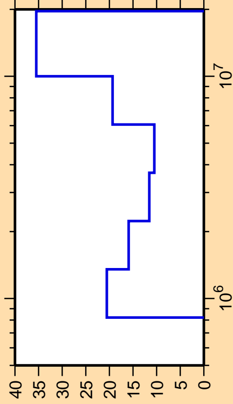
\Delta\sigma/\sigma vs. E for ^{35}\text{Cl}(n,n_1)
