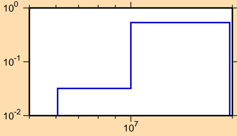
\sigma vs. E for ^{35}\text{Cl}(n,np)
