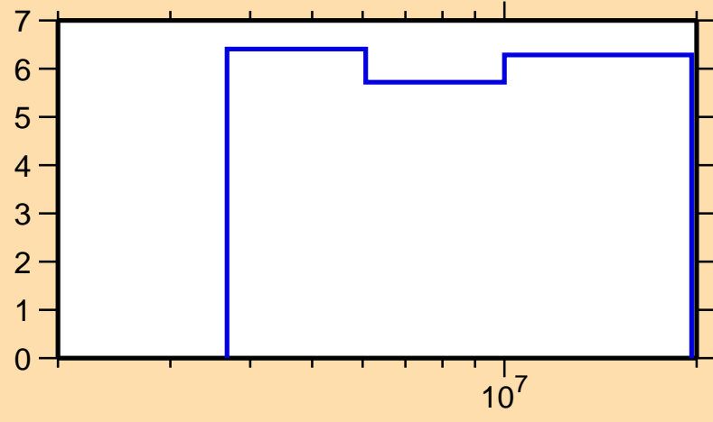
\Delta\sigma/\sigma vs. E for ^{35}\text{Cl}(n,n\text{nonel.})
