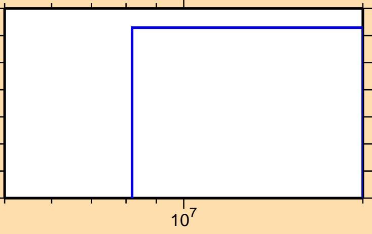
\sigma vs. E for ^{35}\text{Cl}(n,2n)
