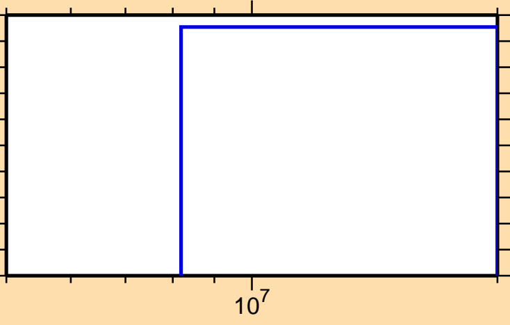
\sigma vs. E for ^{35}\text{Cl}(n,2np)
