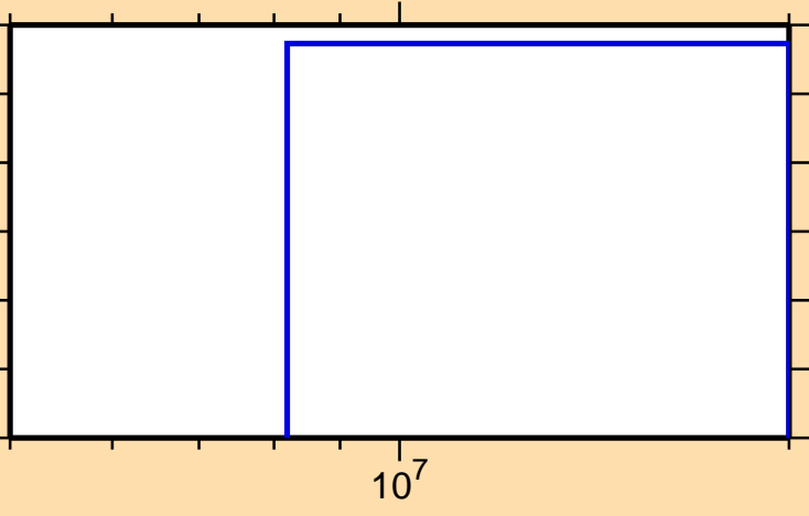
\sigma vs. E for ^{35}\text{Cl}(n,\text{He}3)
