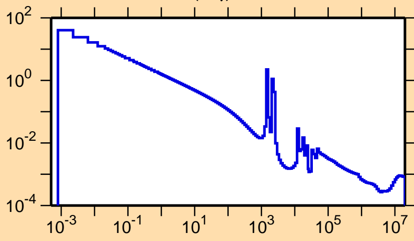
\sigma vs. E for ^{36}\text{Cl}(n,\gamma)
