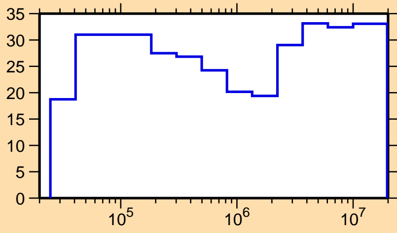
\Delta\sigma/\sigma vs. E for ^{36}\text{Cl}(n,p)
