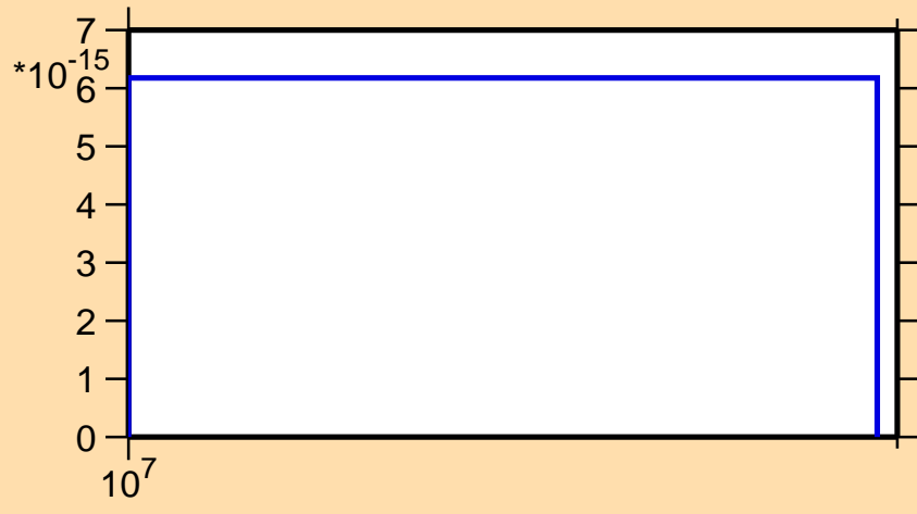
\sigma vs. E for ^{36}\text{Cl}(n,\text{pd})
