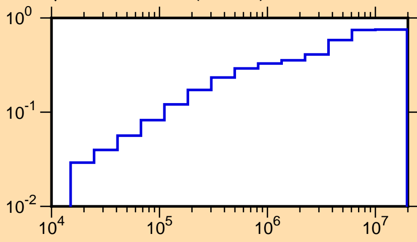
\mu vs. E for ^{37}\text{Cl}(\text{mt251})
