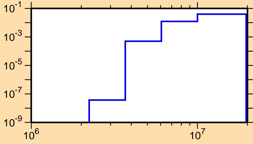
\sigma vs. E for ^{37}\text{Cl}(n,\alpha)
