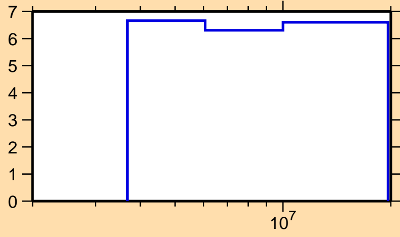
\Delta\sigma/\sigma vs. E for ^{37}\text{Cl}(n, n\text{onel.})
