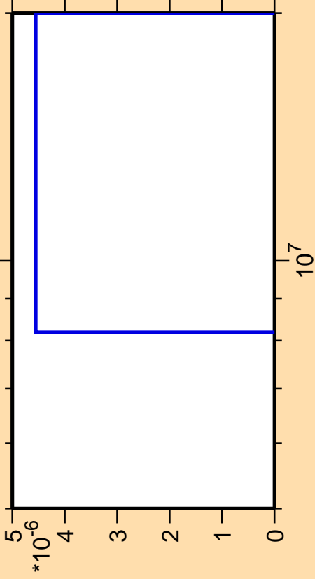
\Delta\sigma/\sigma vs. E for ^{37}\text{Cl} (mt 45)
