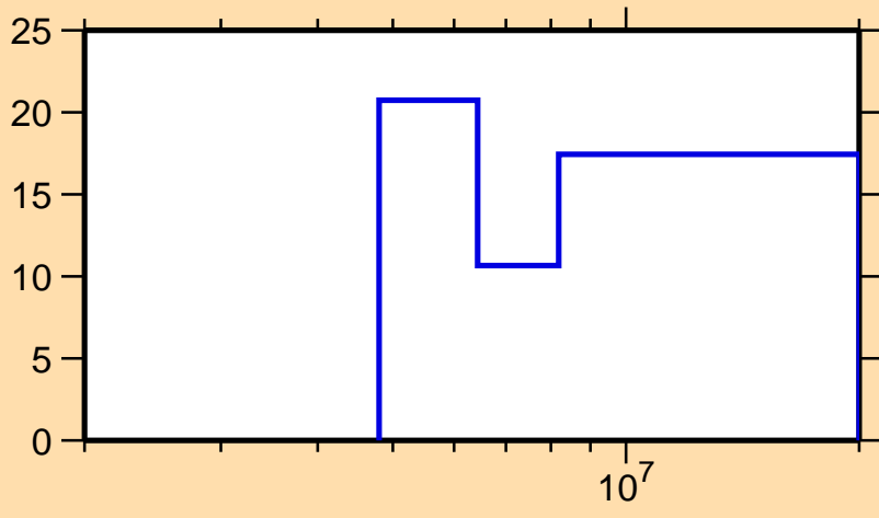
\Delta\sigma/\sigma vs. E for ^{37}\text{Cl}(n,n\text{cont.})
