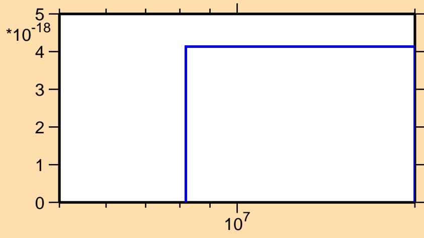
\sigma vs. E for ^{37}\text{Cl} (mt 45)
