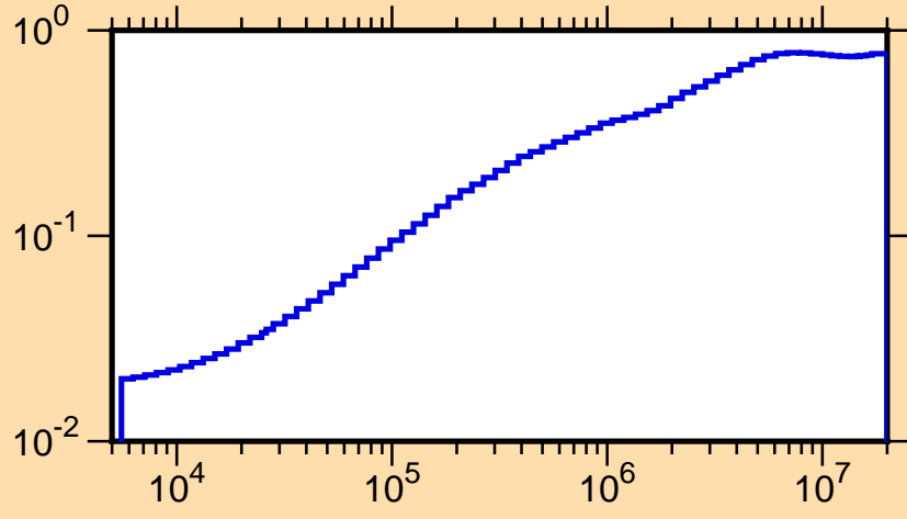
\mu vs. E for ^{38}\text{Cl}(\text{mt251})
