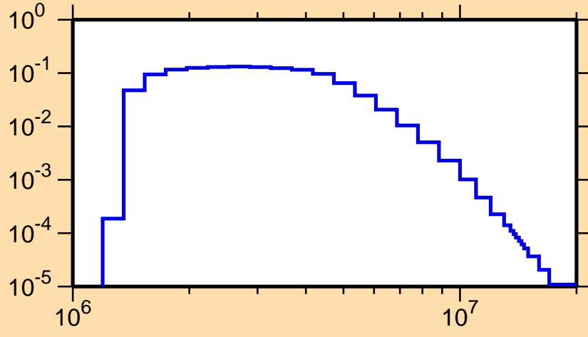
\sigma vs. E for ^{38}\text{Cl}(n,n_3)
