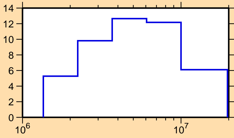
\Delta\sigma/\sigma vs. E for ^{38}\text{Cl}(n,el.)
