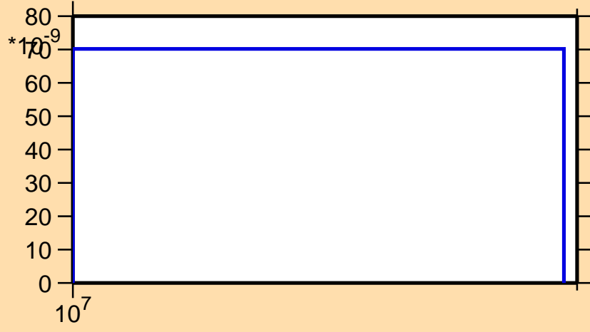
\sigma vs. E for ^{38}\text{Cl}(n,nt)
