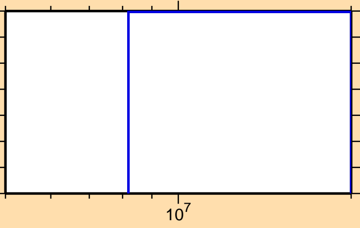
\sigma vs. E for ^{38}\text{Cl}(n,\text{nd})
