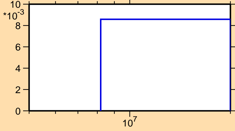
\sigma vs. E for ^{38}\text{Cl}(n,n\alpha)
