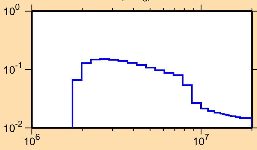
\sigma vs. E for ^{39}\text{Cl}(n,n_3)
