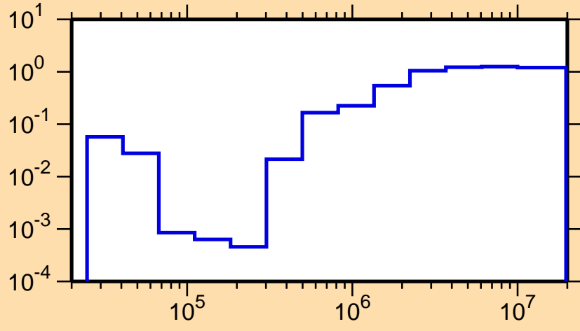
\sigma vs. E for ^{39}\text{Cl}(n,\text{nonel.})
