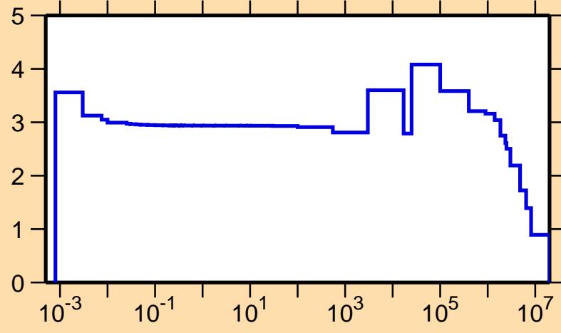
\sigma vs. E for ^{39}\text{Cl}(n,\text{el.})
