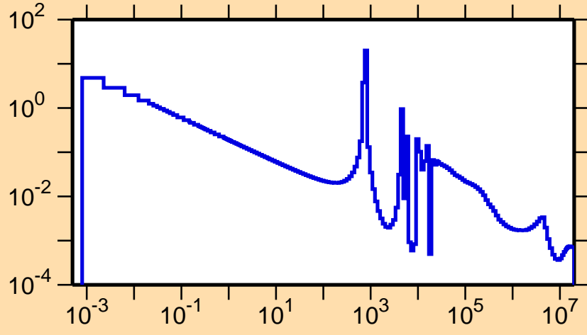
\sigma vs. E for ^{40}\text{Cl}(n,\gamma)
