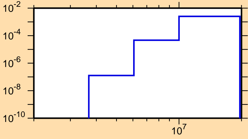
\sigma vs. E for ^{40}\text{Cl}(n,\alpha)
