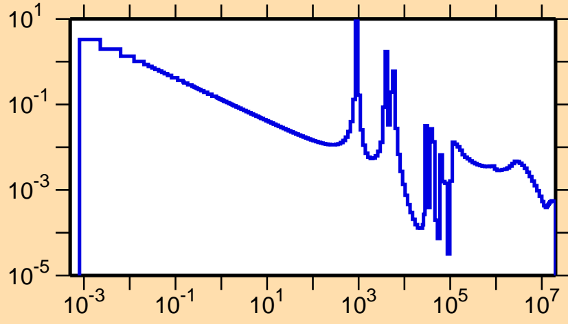
\sigma vs. E for ^{41}\text{Cl}(n,\gamma)
